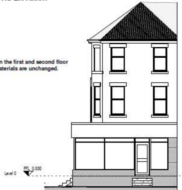
Main St Elevation 1 : 100
