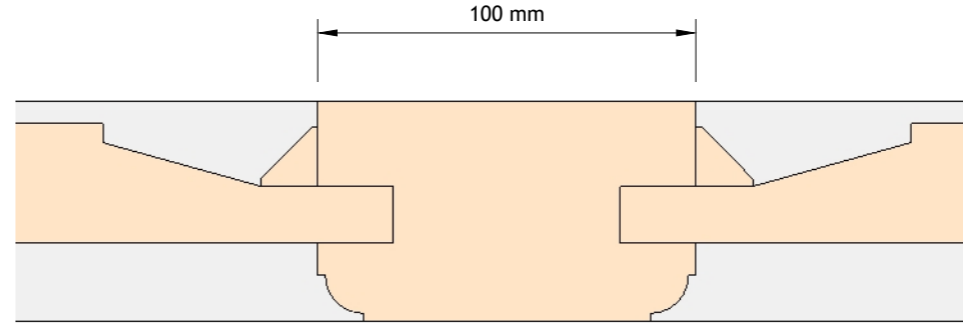
I-GPD-07 Inward Opening Glazed Panelled Door Lower Mullion
