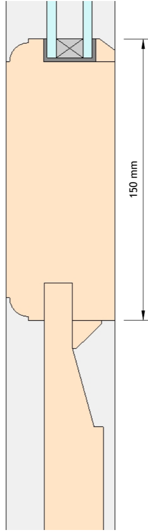
I-GPD-06 Inward Opening Glazed Panelled Door Intermediate Rail
