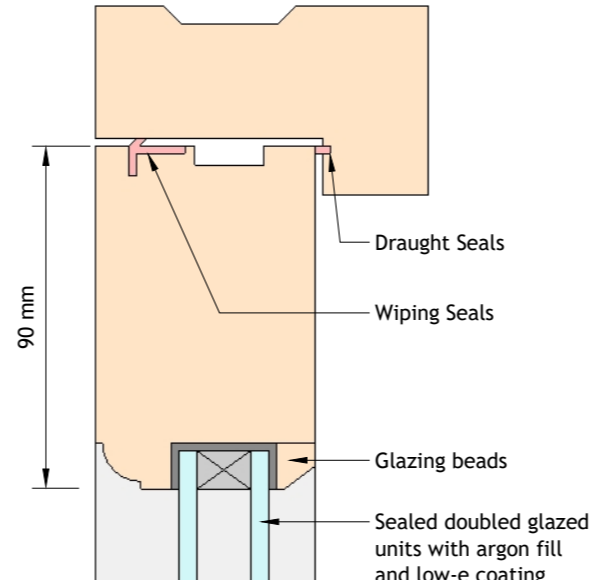
I-GPD-01 Inward Opening Glazed Panelled Door Head
