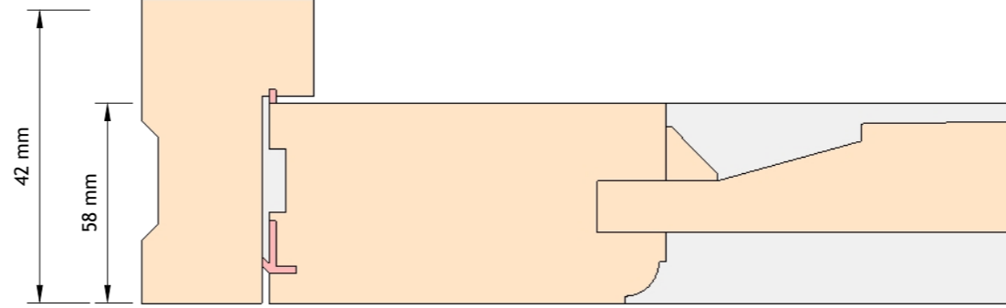
I-GPD-04 Inward Opening Glazed Panelled Door Lower Jamb
