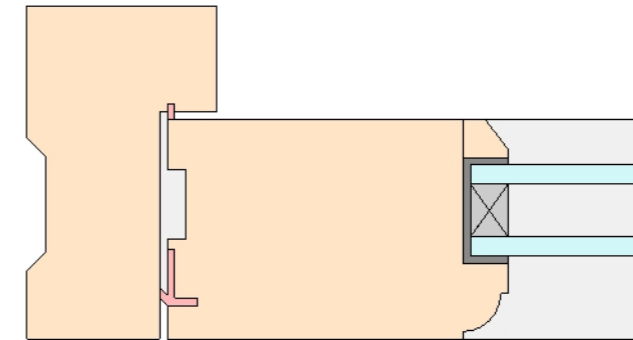
I-GPD-03 Inward Opening Glazed Panelled Door Upper Jamb
