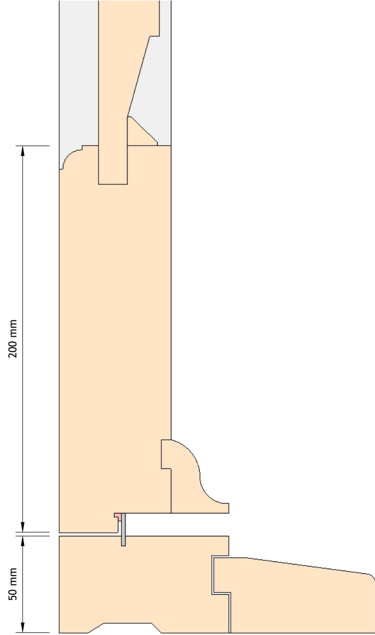
I-GPD-01 Inward Opening Glazed Panelled Door Threshold
