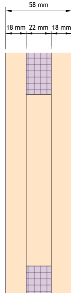
O-FLBD-06 Outward Opening Framed, Ledged and Boarded Door Intermediate Rail
