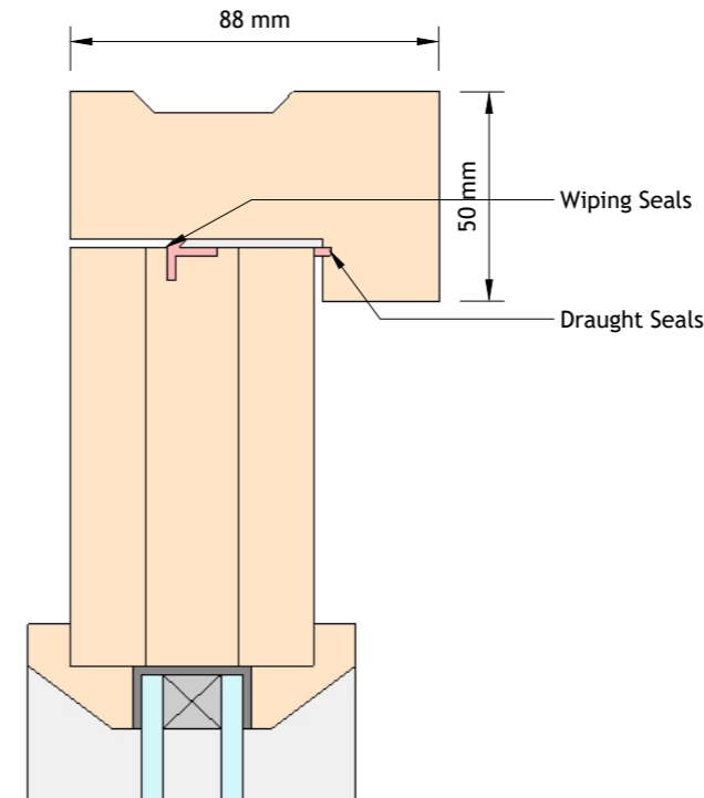
O-FLBD-02 Outward Opening Framed, Ledged and Boarded Door Head
