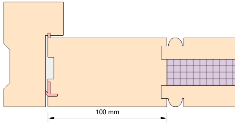
O-FLBD-03 Outward Opening Framed, Ledged and Boarded Door Jamb
