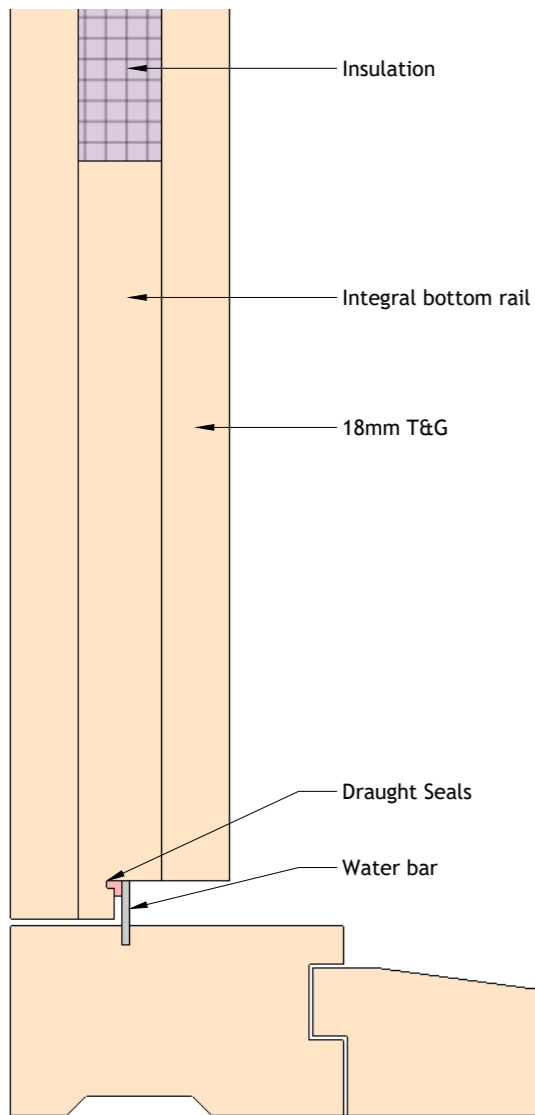
O-FLBD-01 Outward Opening Framed, Ledged and Boarded Door Threshold
