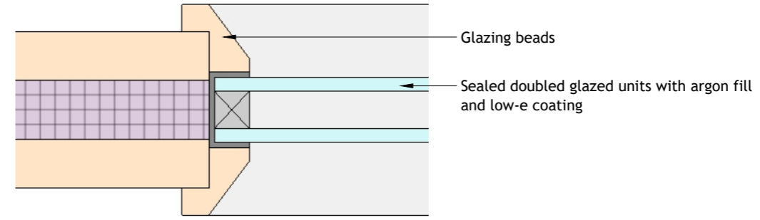
O-FLBD-07 Outward Opening Framed, Ledged and Boarded Door Doorlite
