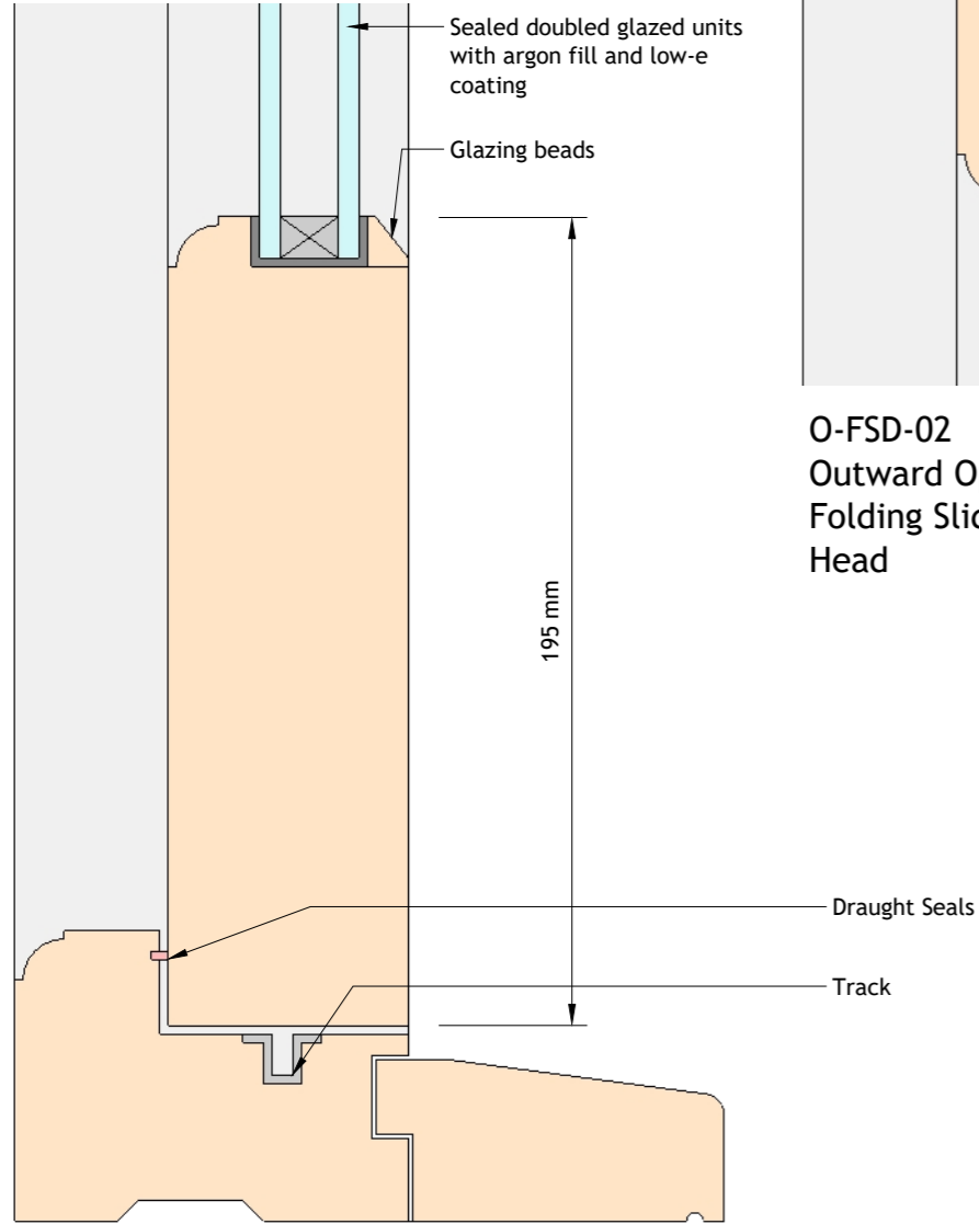
O-FSD-01 Outward Opening Folding Sliding Door Threshold
