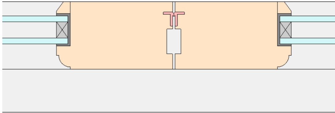
O-FSD-05 Outward Opening Folding Sliding Door Fold
