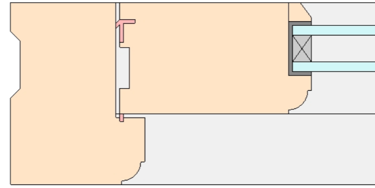
O-FSD-03 Outward Opening Folding Sliding Door Jamb
