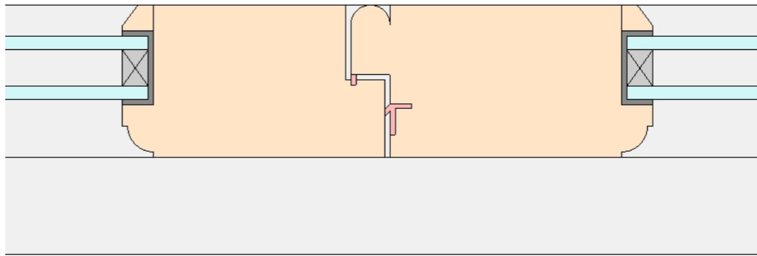
O-FSD-04 Outward Opening Folding Sliding Door Rebate
