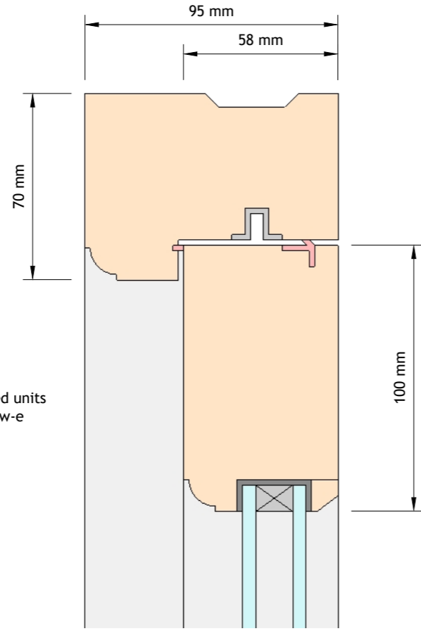
O-FSD-02 Outward Opening Folding Sliding Door Head
