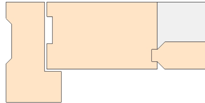
O-FLBBD-03 Outward Opening Framed, Ledged, Braced and Boarded Door Jamb
