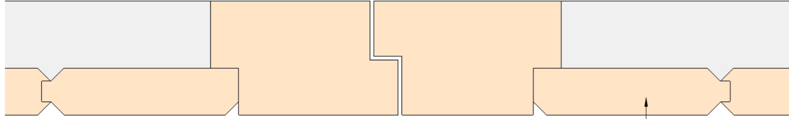
O-FLBBD-04 Outward Opening Framed, Ledged, Braced and Boarded Door Meeting Style
