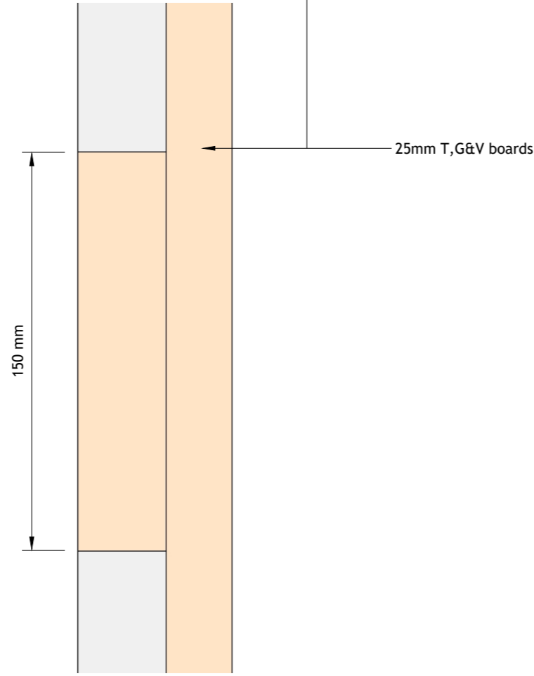
O-FLBBD-06 Outward Opening Framed, Ledged, Braced and Boarded Door Intermediate Rail
