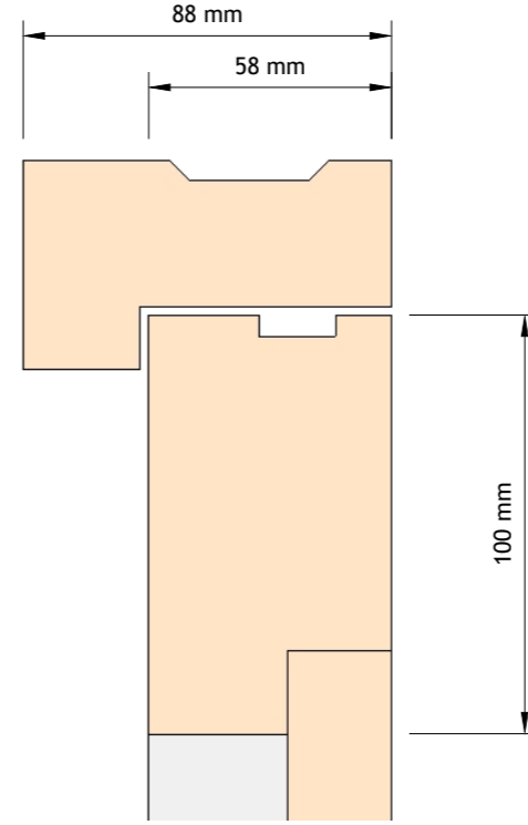
O-FLBBD-02 Outward Opening Framed, Ledged, Braced and Boarded Door Head
