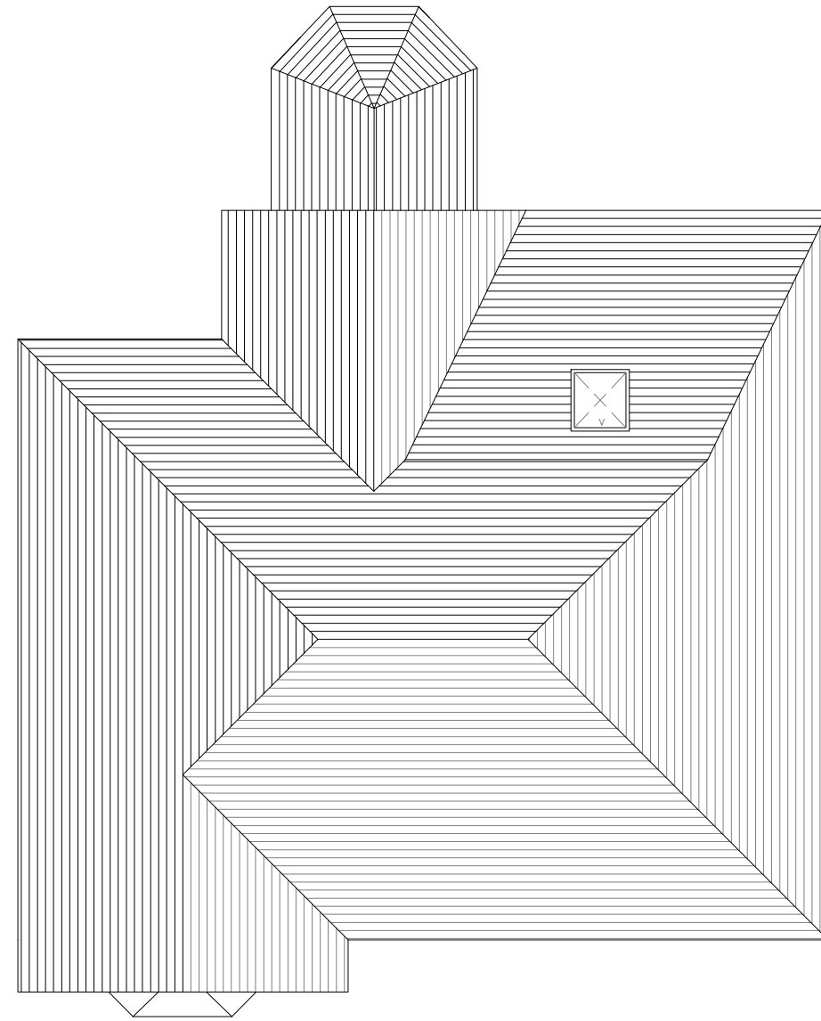
Roof Plan
