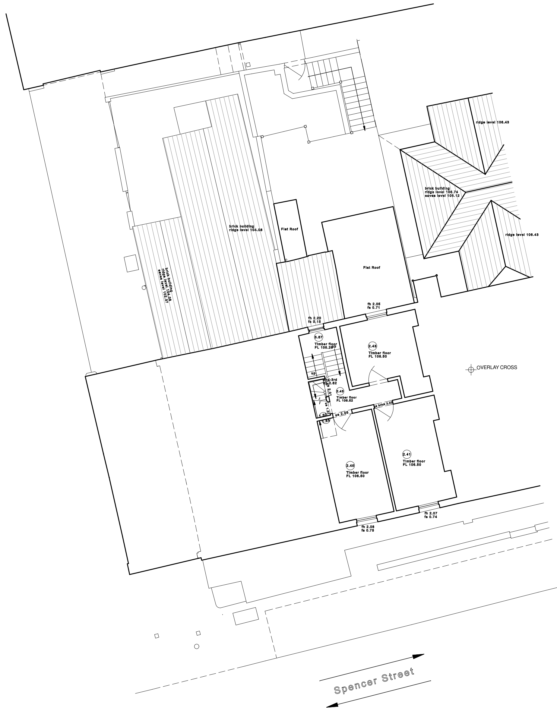
EXISTING SECOND FLOOR PLAN
