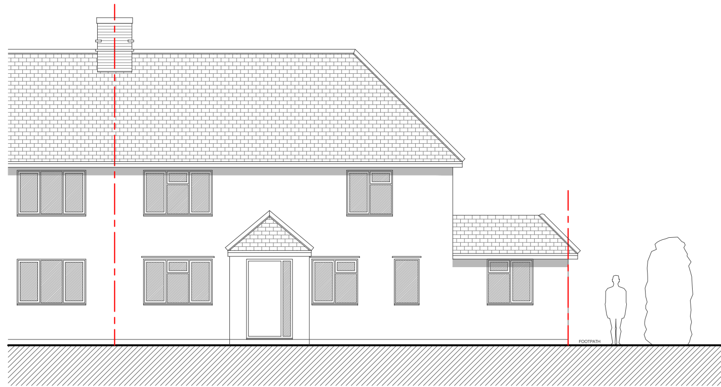
existing drawing WEST ELEVATION
