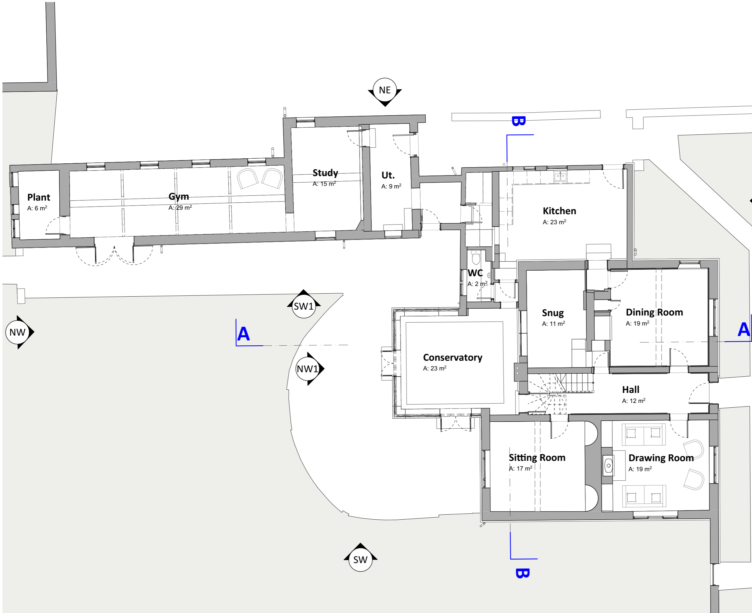
Existing Ground Floor 1:100
