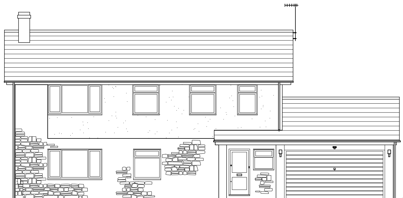
Existing South Elevations
