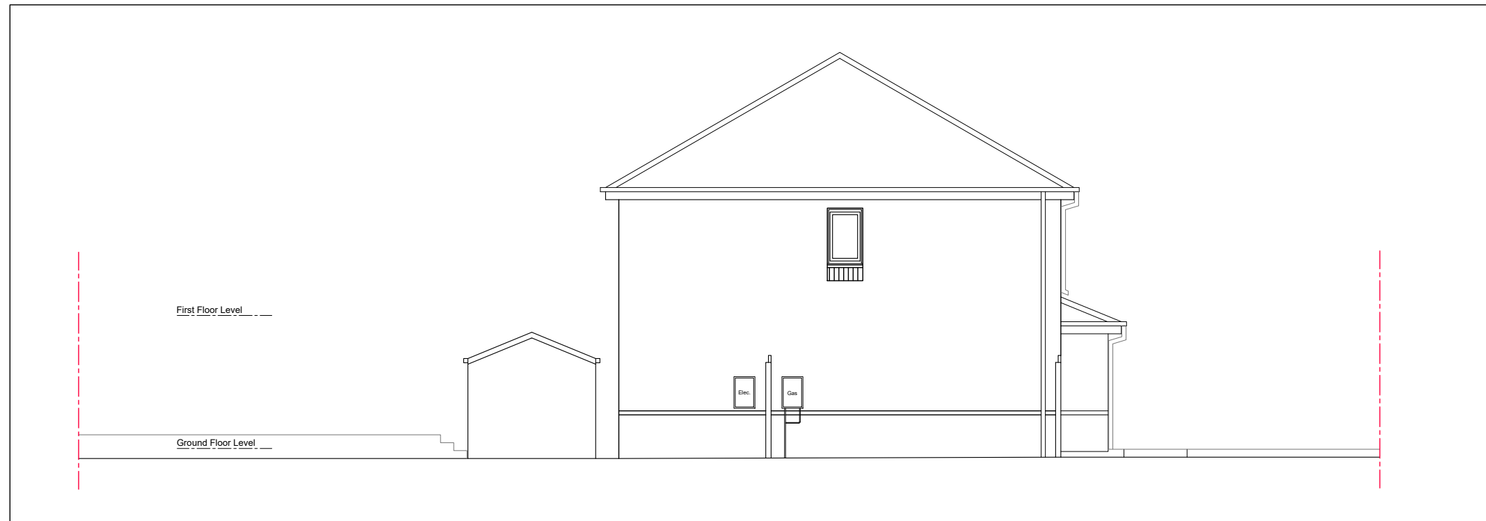
West (Side) Elevation as Existing @ 1:100
