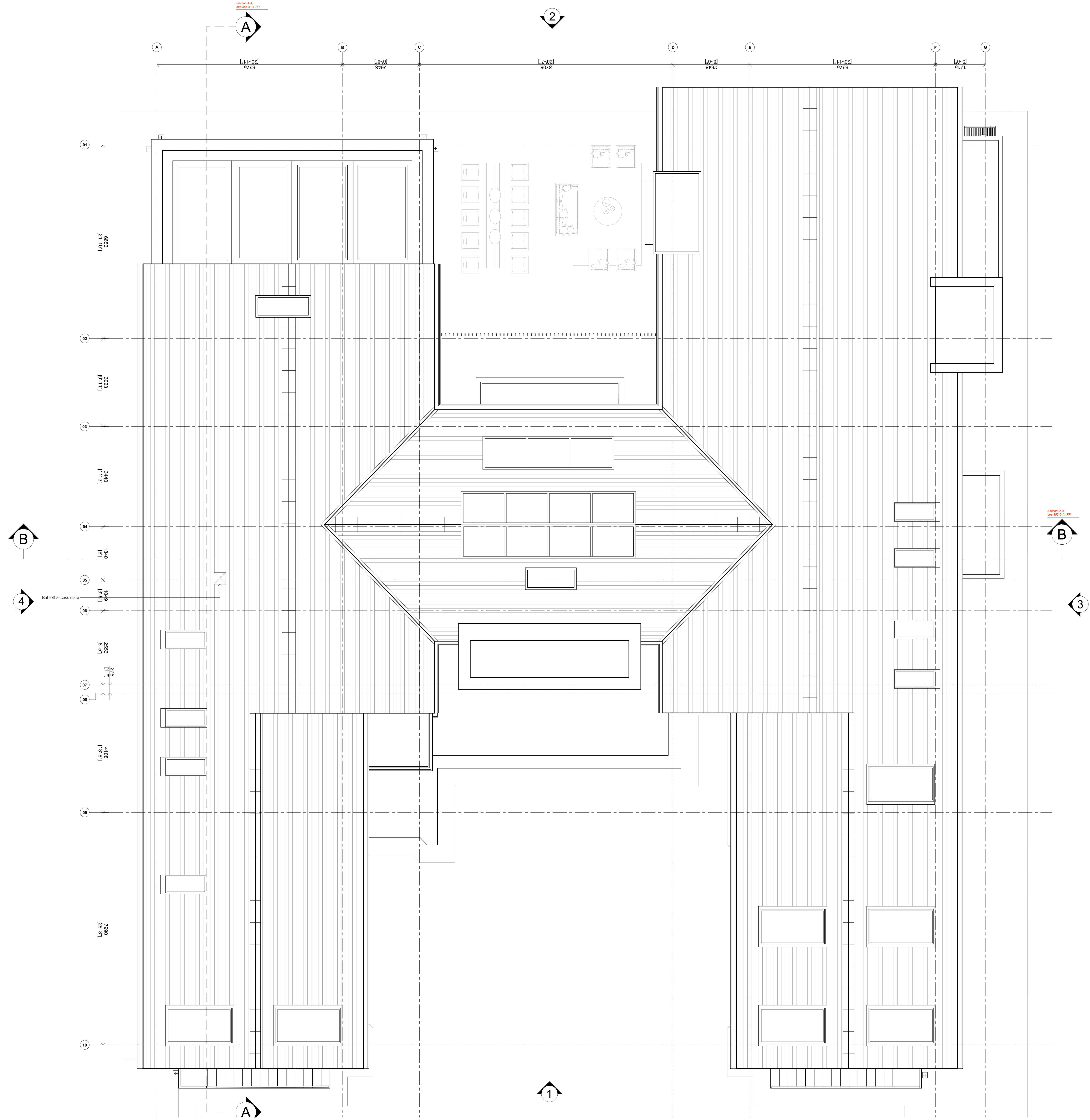
Roof Plan as 'Proposed' Scale 1:50
