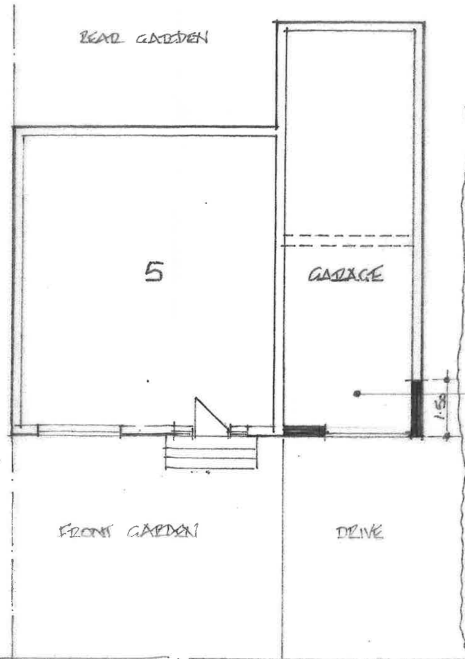
EXISTING GROUND FLOOR PLAN / BLOCK PLAN. PROPOSED GROUND FLOOR / BLOCK PLAN
