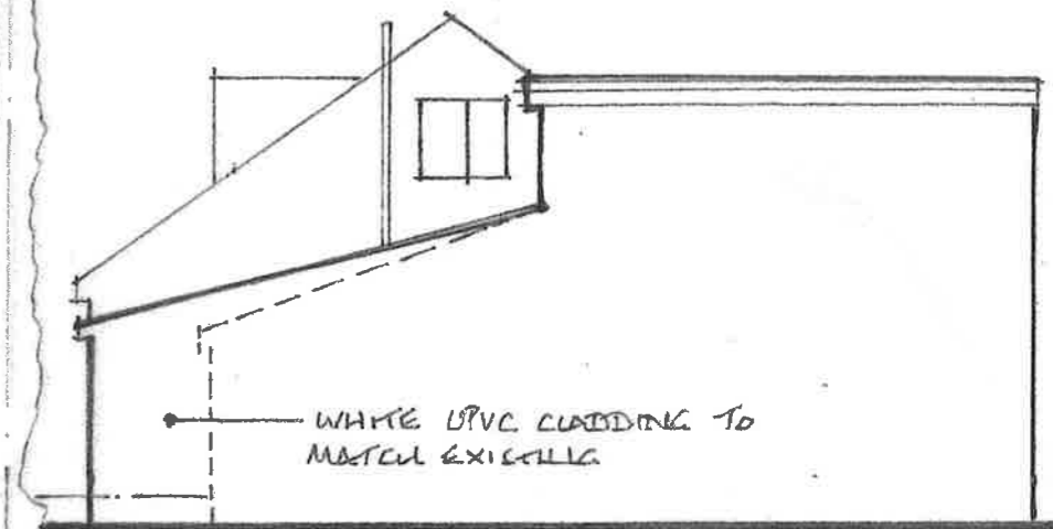
PROPOSED EXTENSION? PROPOSED SIDE ELEVATION
