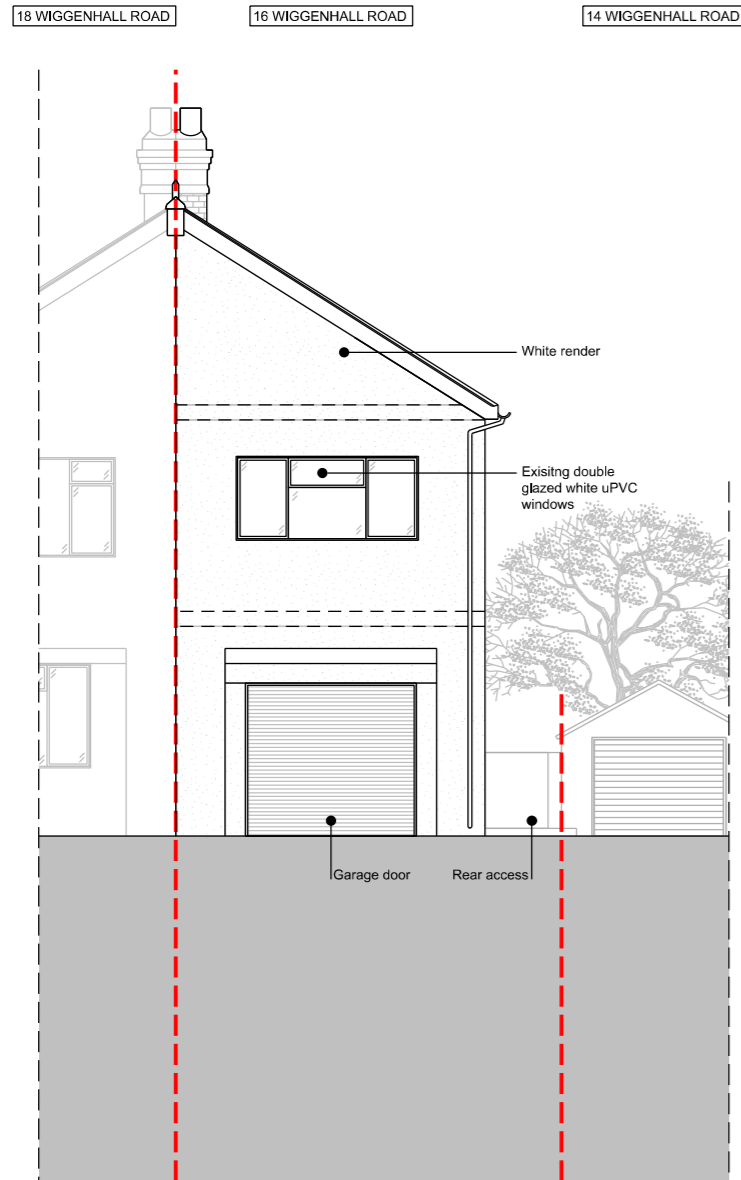
01 EXISTING FRONT ELEVATION 1:100@A3
