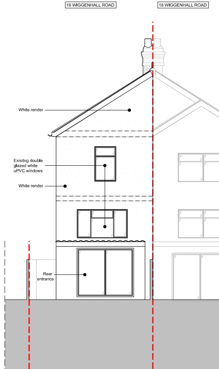
02 EXISTING REAR ELEVATION 1:100@A3
