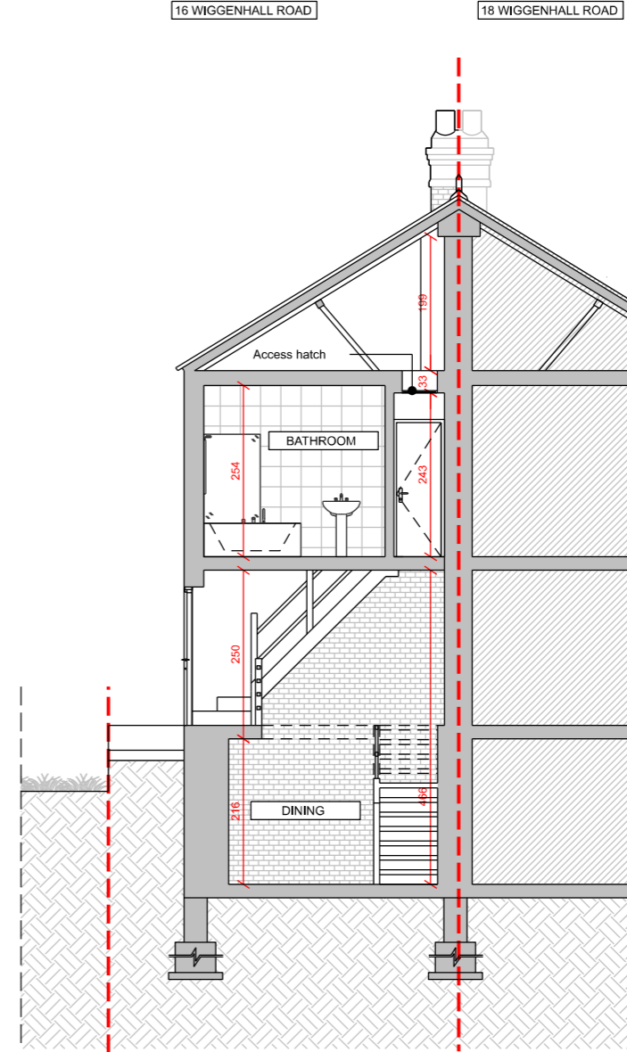
03 EXISTING CROSS SECTION 1:100@A3
