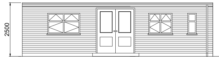
Front Elevation 1:100
