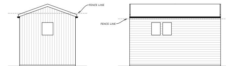
EXISTING ELEVATIONS (SHED A) 1:100
