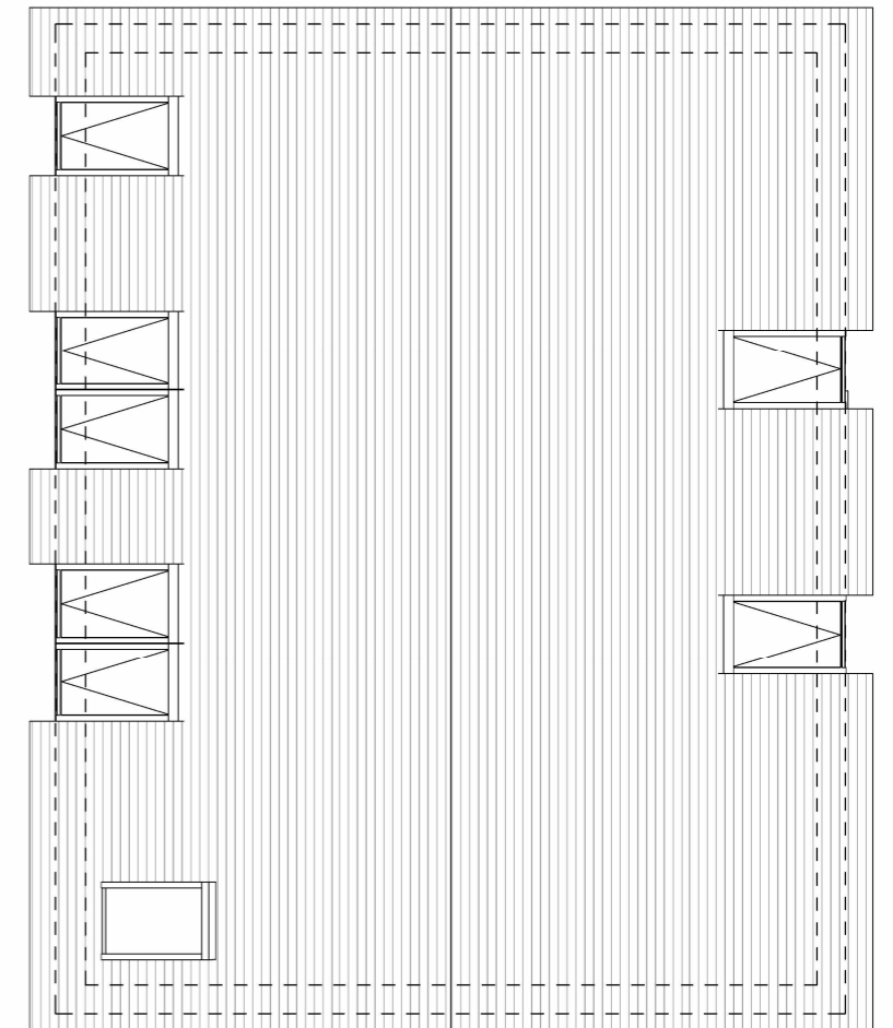
Roof Plan as Proposed 1 : 100
