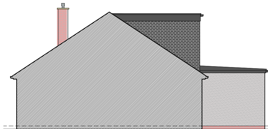
4. Proposed South Elevation Scale 1:100
