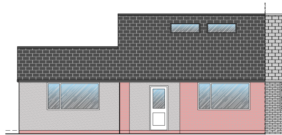
2. Proposed West Elevation Scale 1:100
