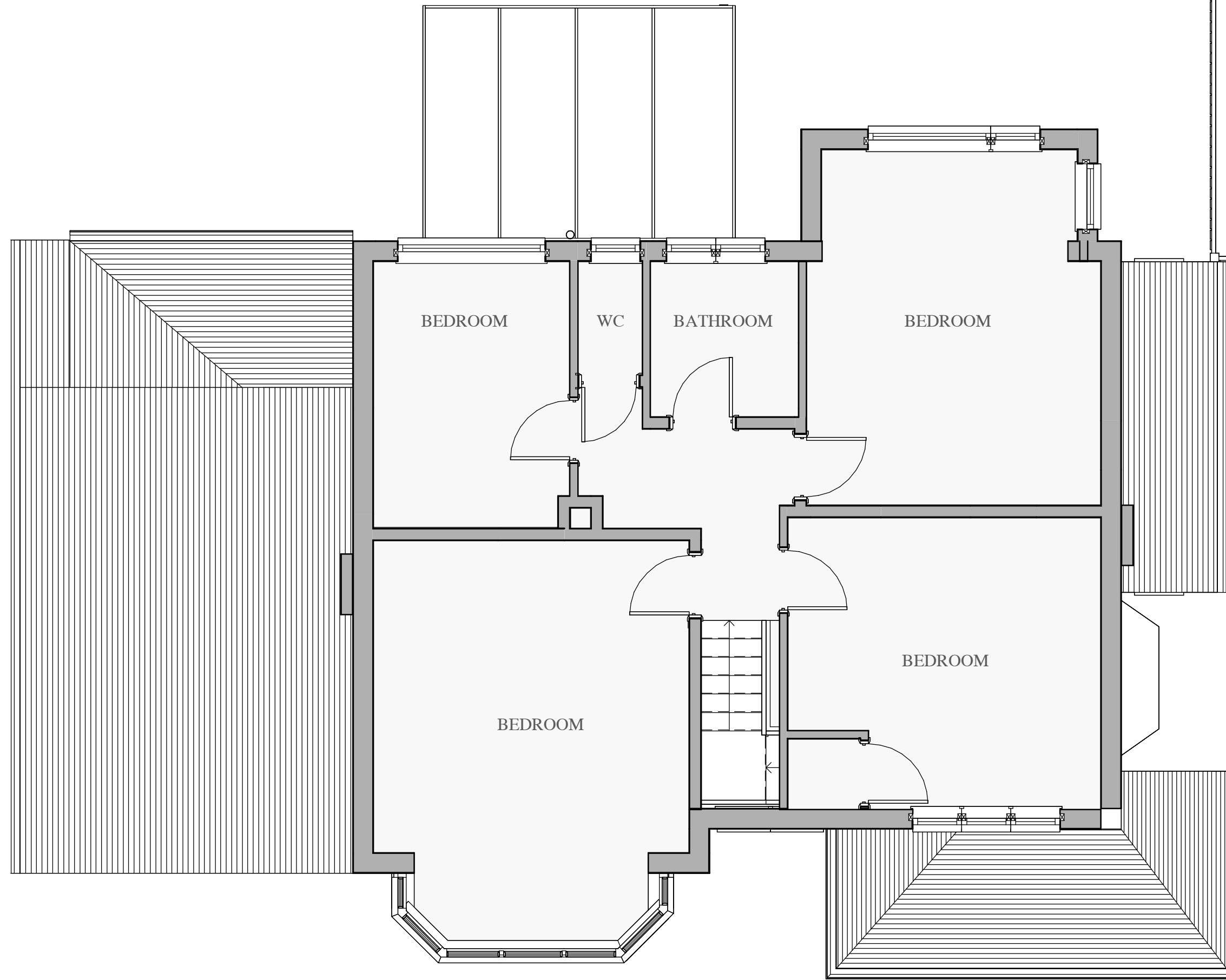
02 Existing First Floor 1 : 50
