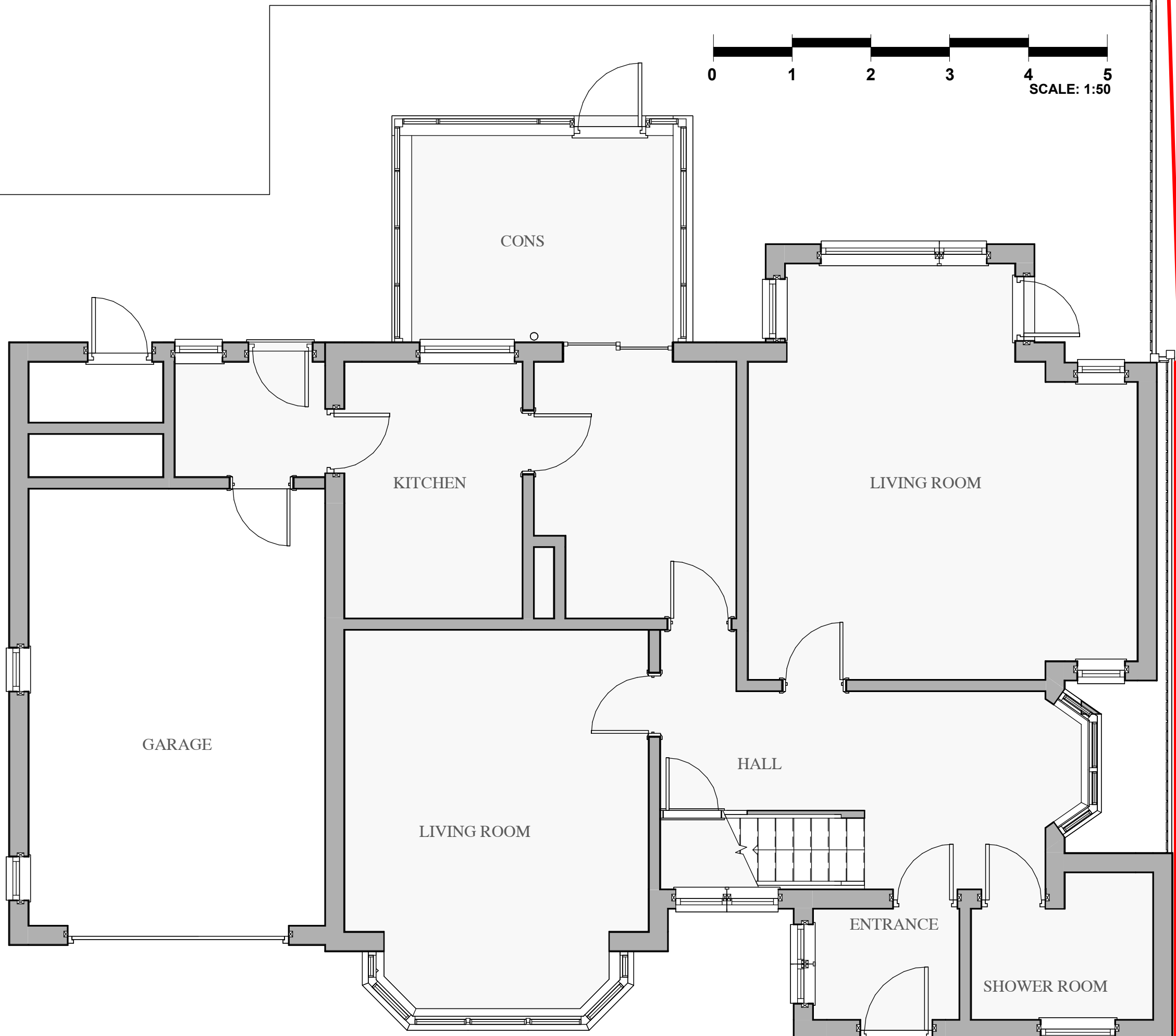
01 Existing Ground Floor 1 : 50
