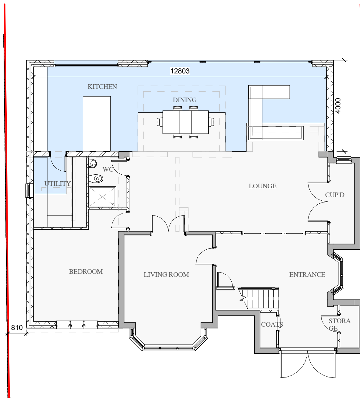
01 Proposed Ground Floor 1 : 100
