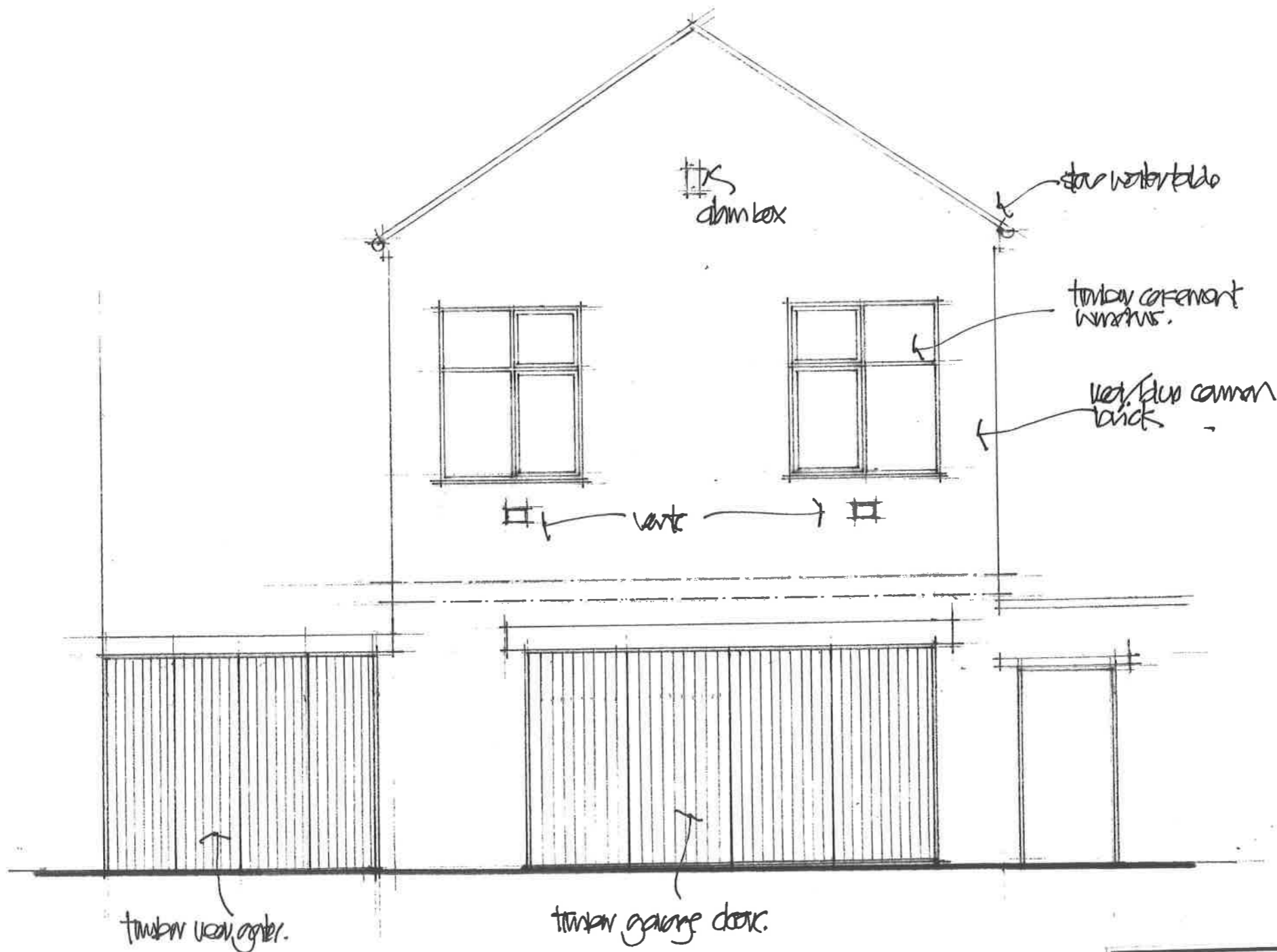
Rear Elevation
