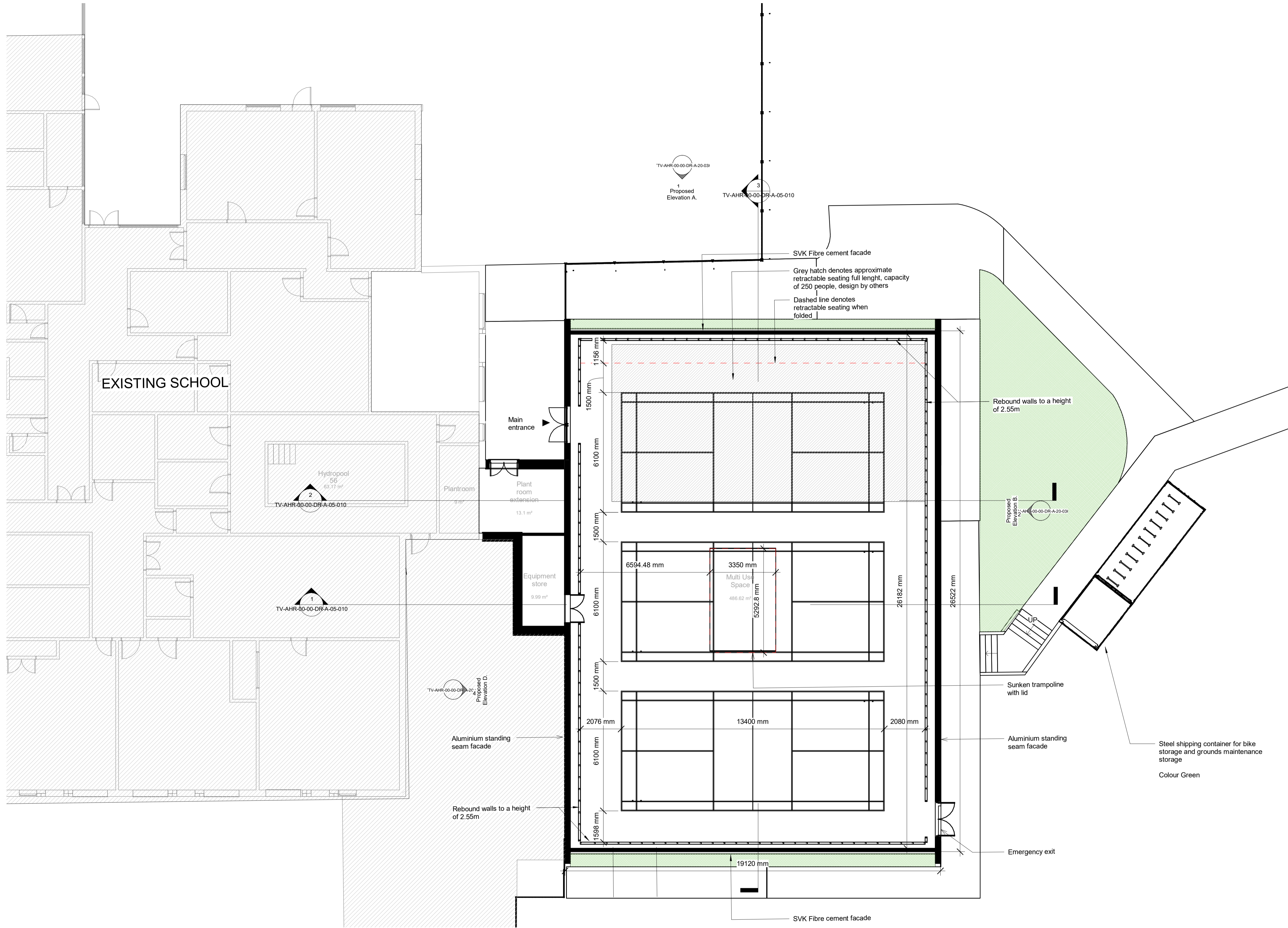
1 Multi Use Space Proposed General Arrangement 1:100
