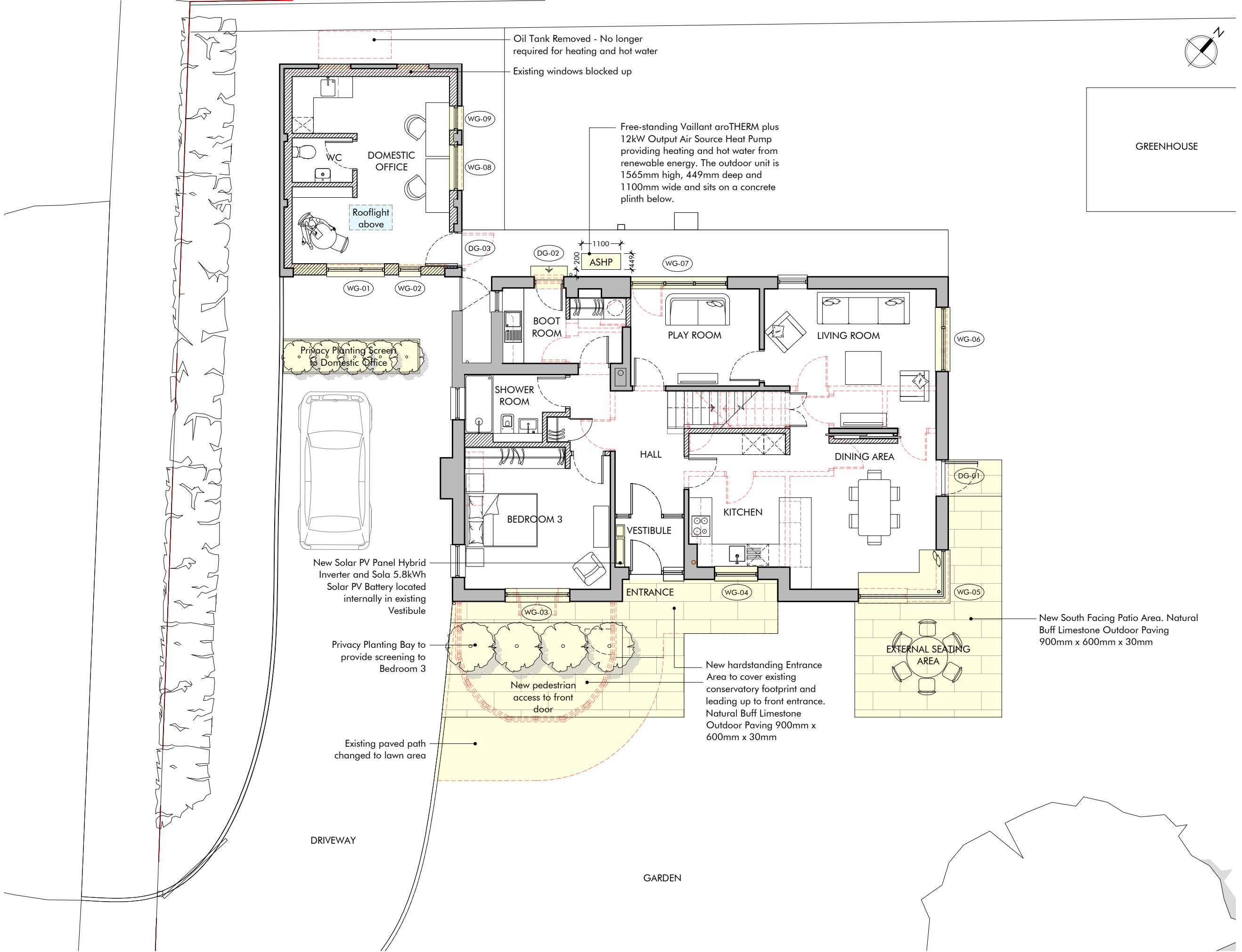
PROPOSED GROUND FLOOR PLAN SCALE 1:100 @ A3
