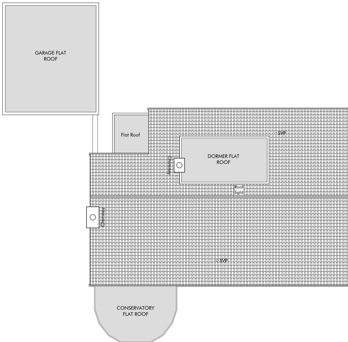
EXISTING ROOF PLAN SCALE 1:100 @ A3
