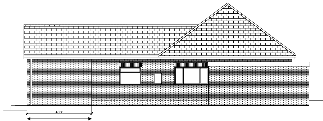
Side elevation 4 meter Single storey extension To match existing red clay brick and clay roof tile
