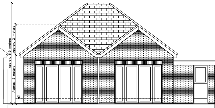
Rear elevation 4 meter single storey extension To match existing red clay brick and clay roof tile
