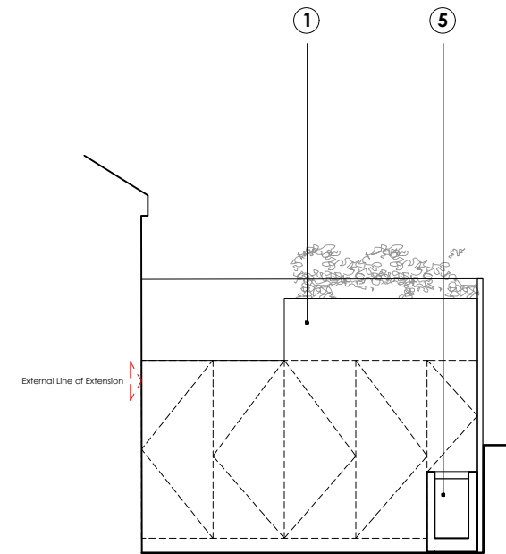
Elevation CC
