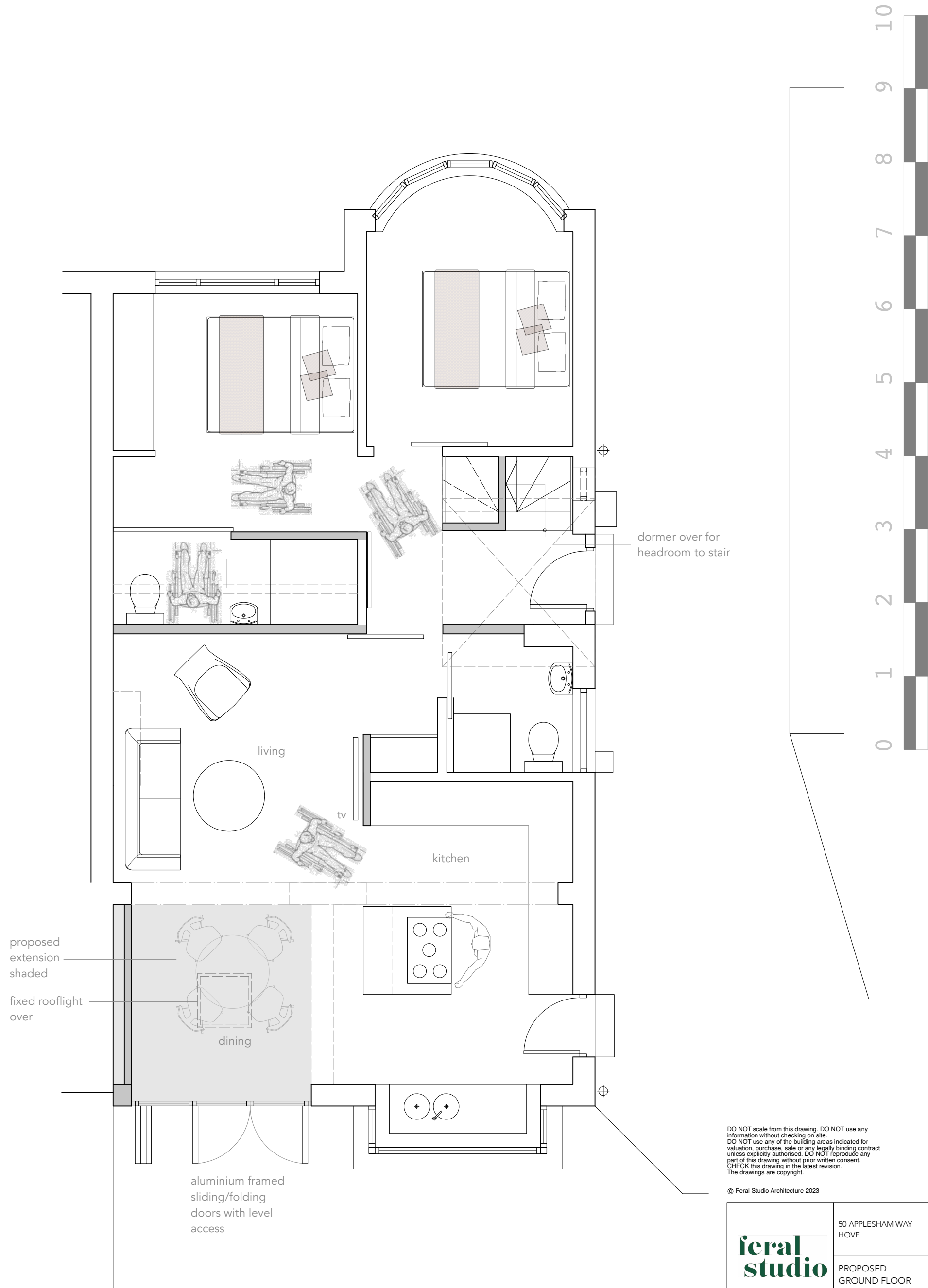
1 GROUND FLOOR PLAN PROPOSED
