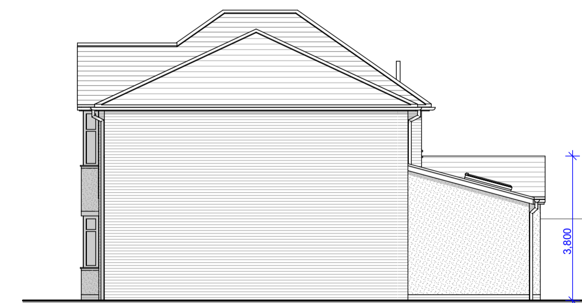
Proposed Side Elevation [South West] Scale: 1:100
