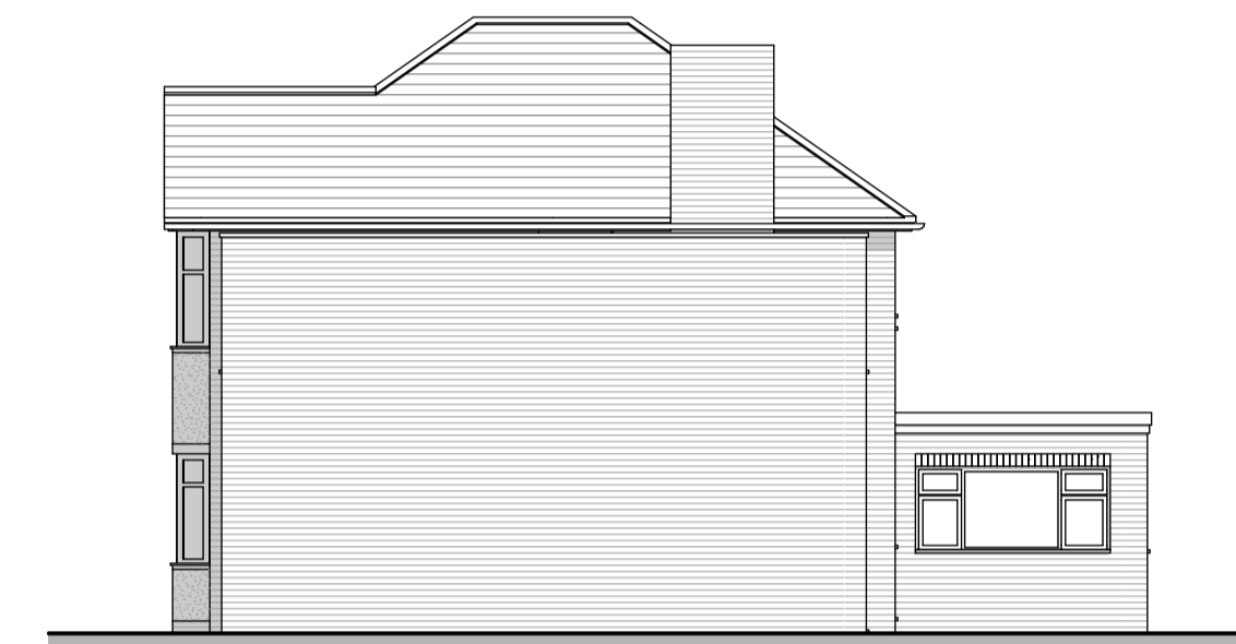
Existing Side Elevation [South West] Scale: 1:100
