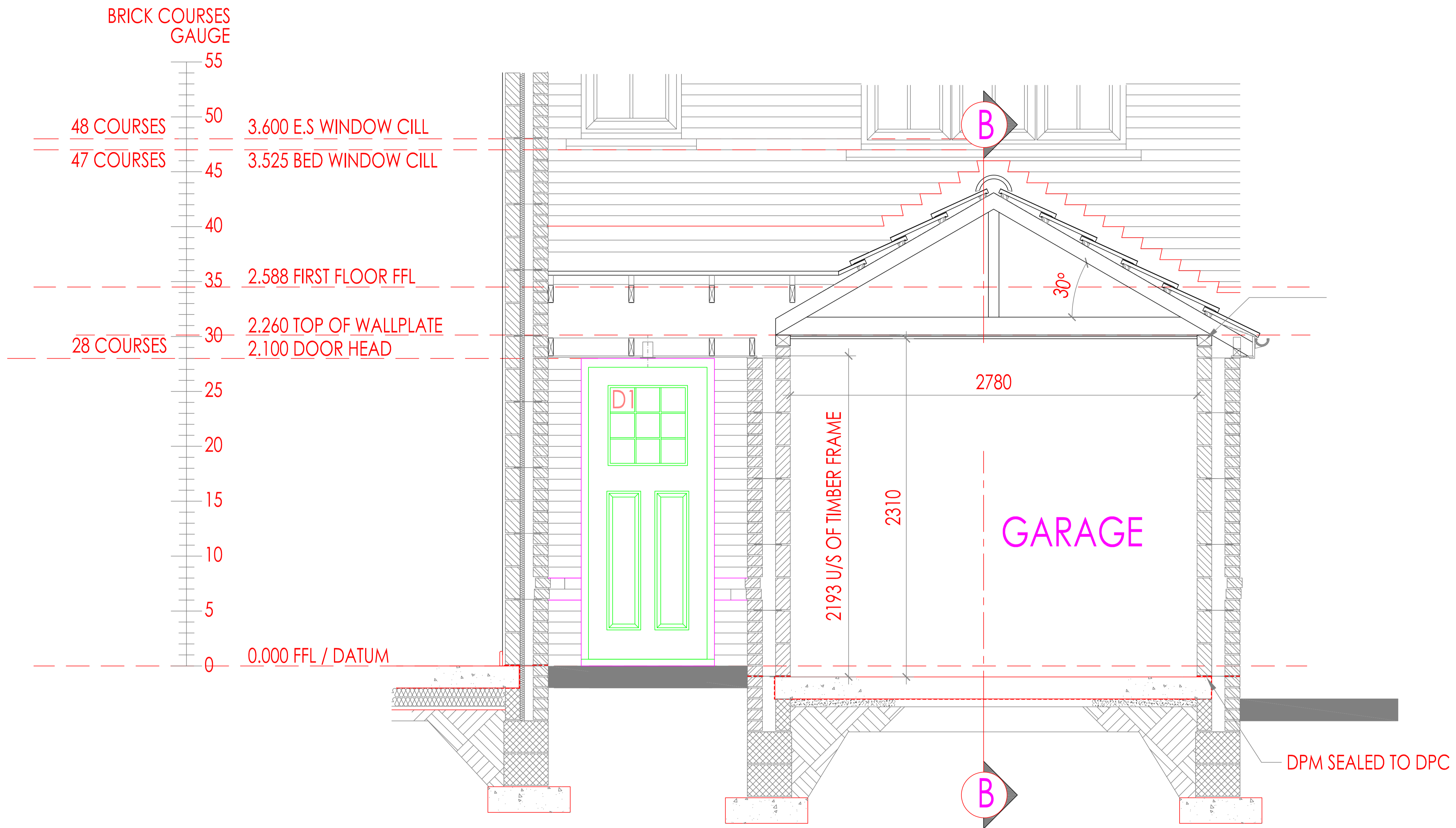
SECTION C-C
