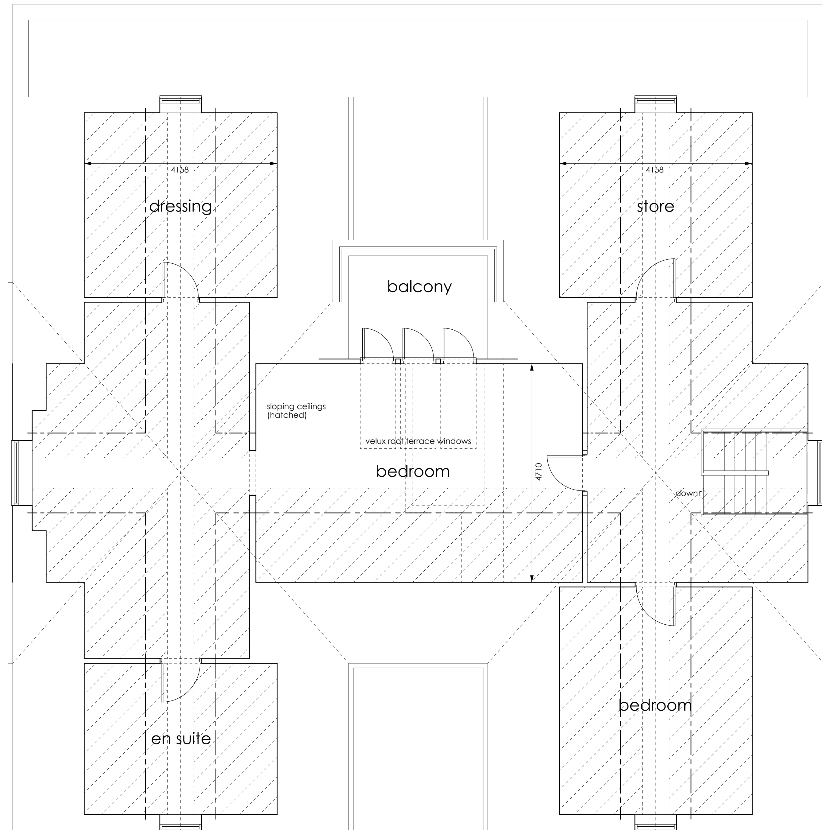
ROOF PLAN
