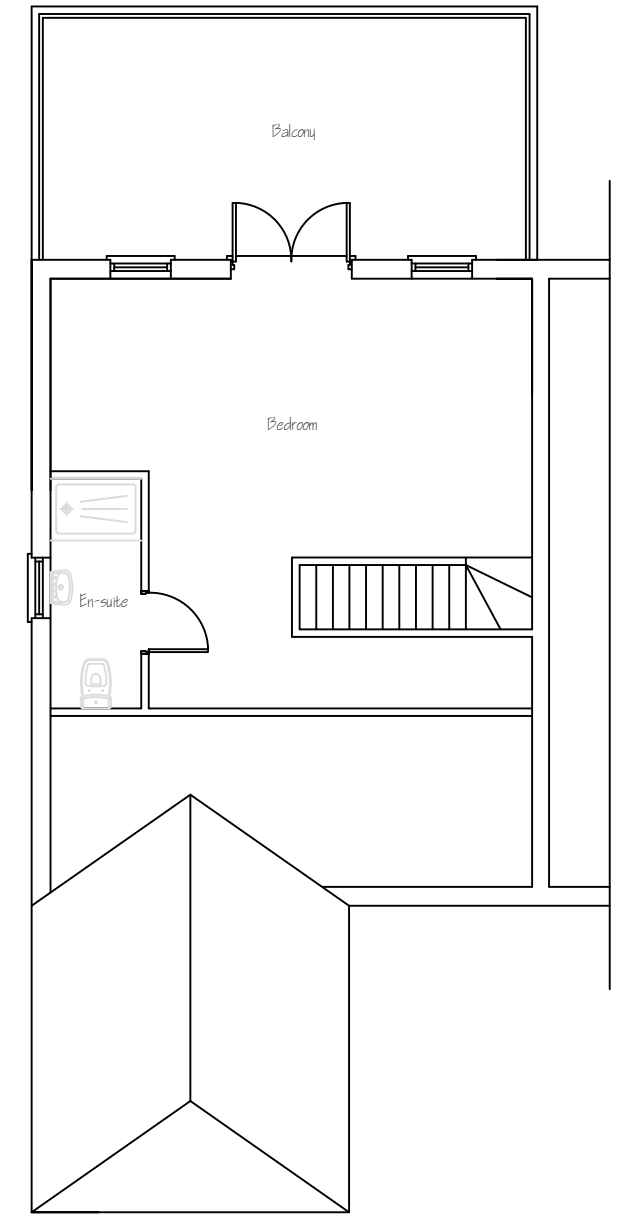
PROPOSED FIRST FLOOR LAYOUT
