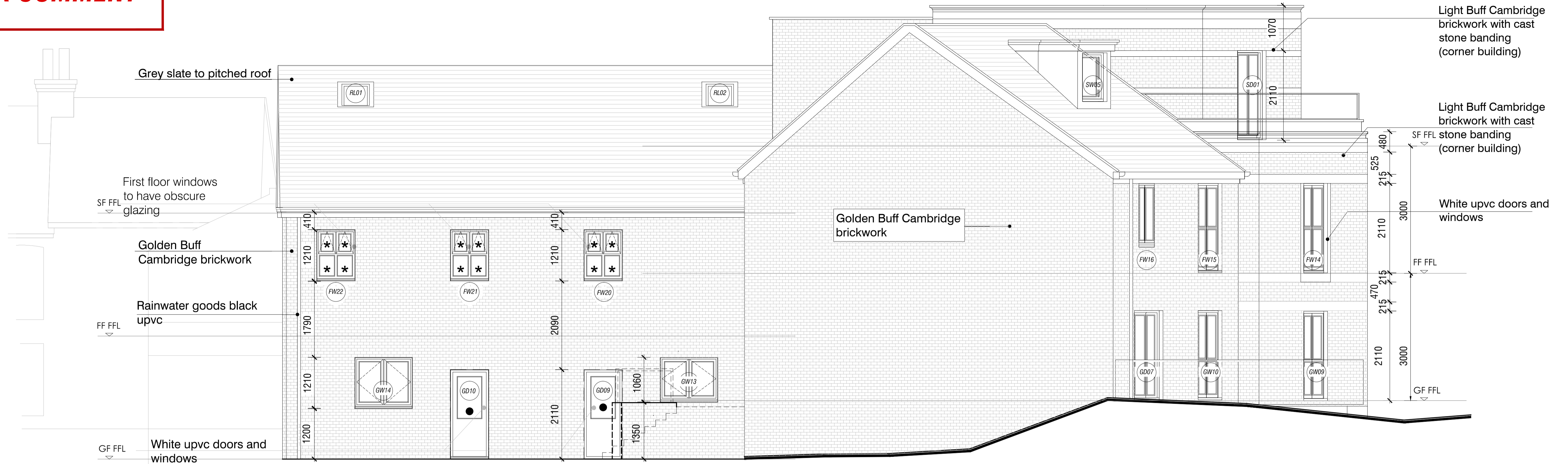
PROPOSED ELEVATION SOUTH EAST (REAR) Proposed | 1:100
