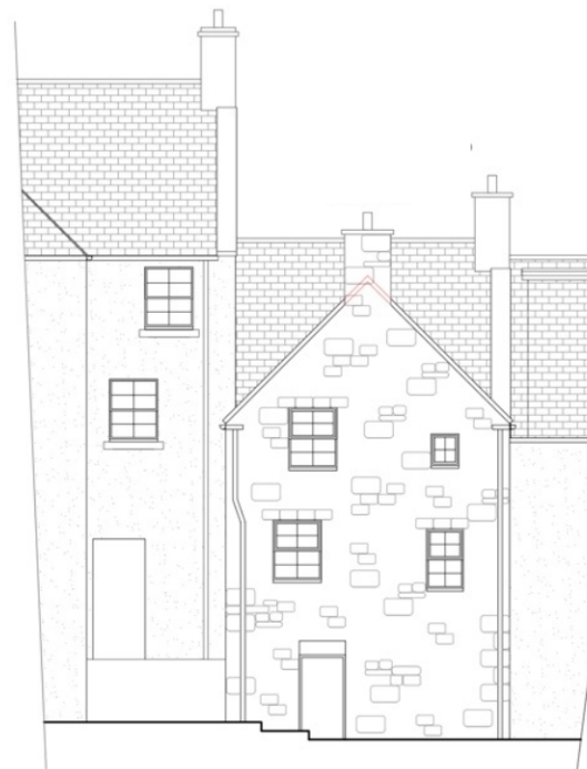
South-West Elevation 1:100
