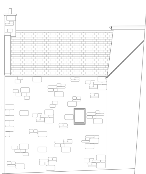
South-East Elevation 1:100
