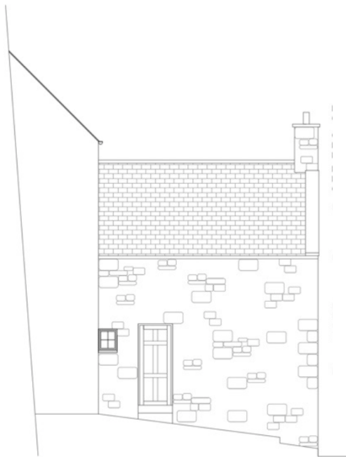
North-West Elevation 1:100
