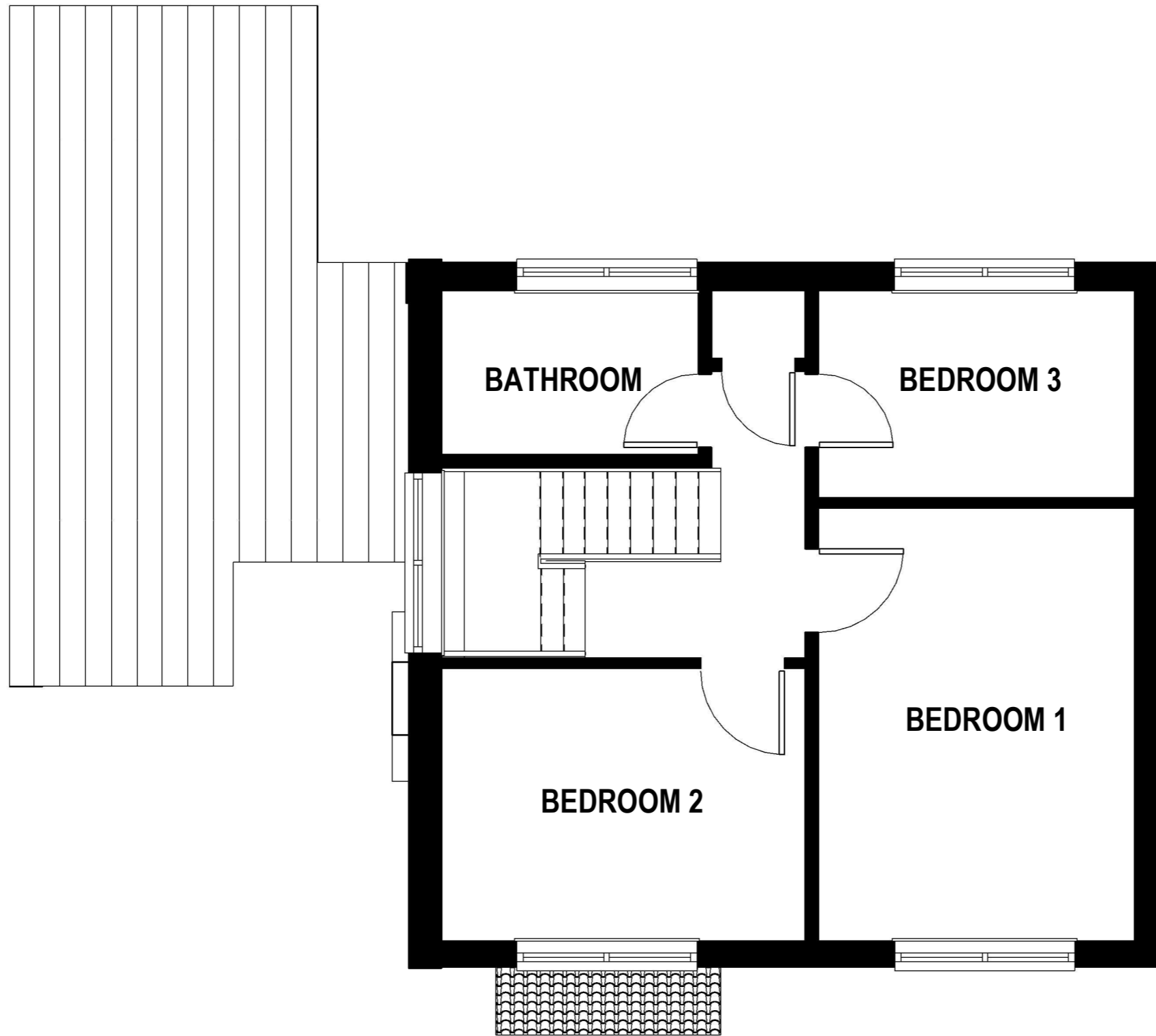
1 -Existing First floor plan 1 : 50
