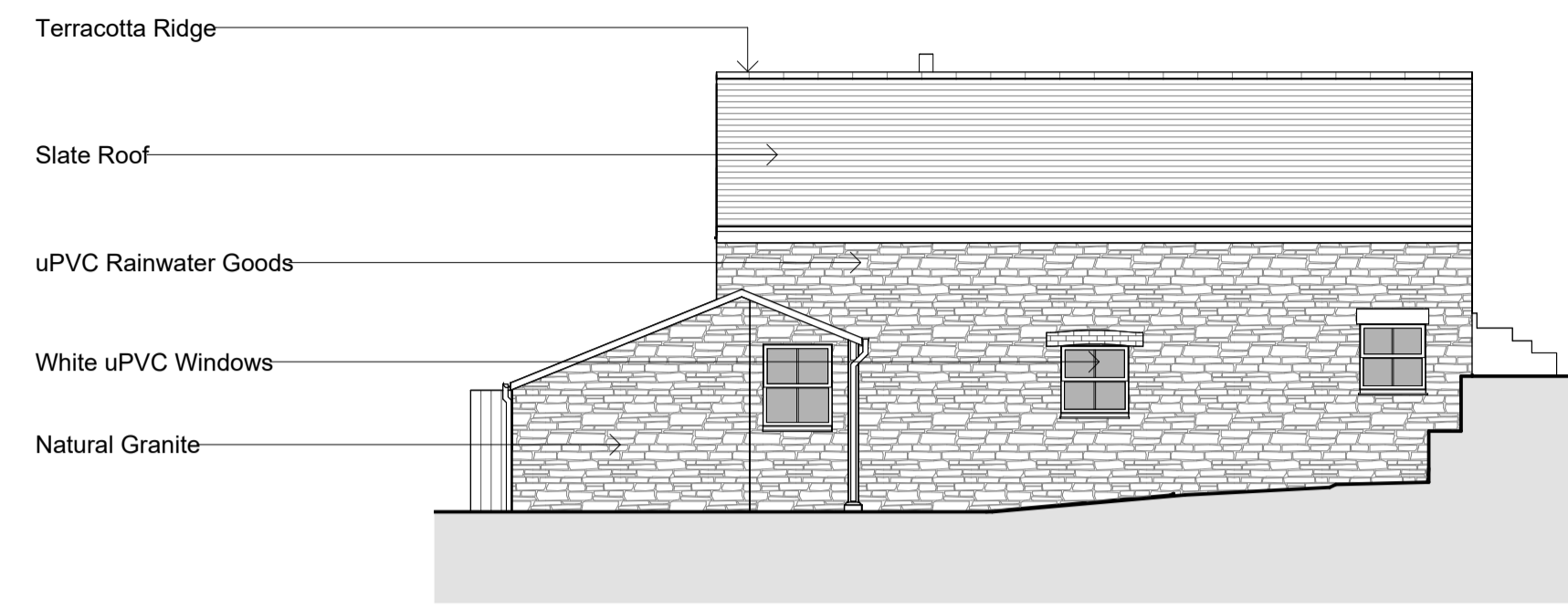
1 Elevation 1 - South West Elevation 1 : 100
