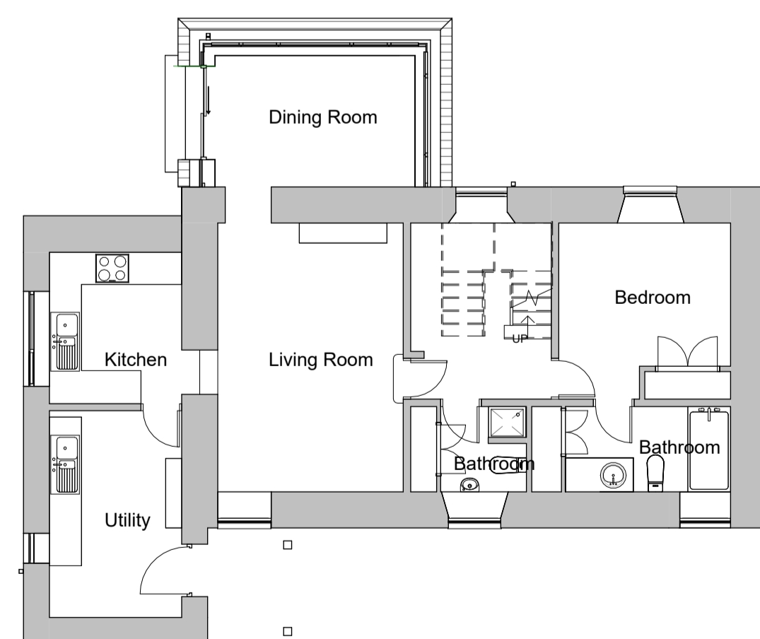
5 Ground Floor 1 : 100
