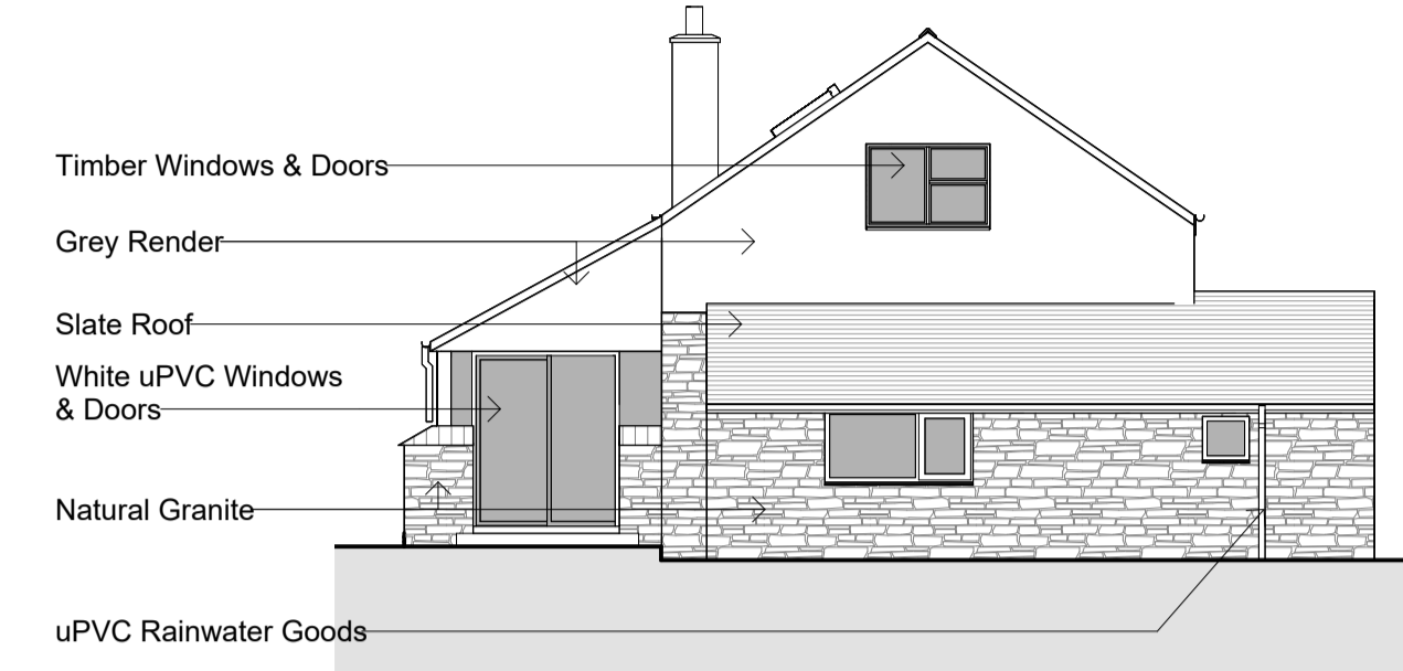
2 Elevation 2 - North West Elevation 1 : 100
