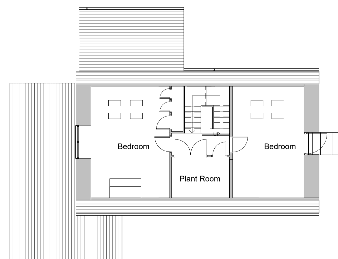
6 First Floor Plan 1 : 100
