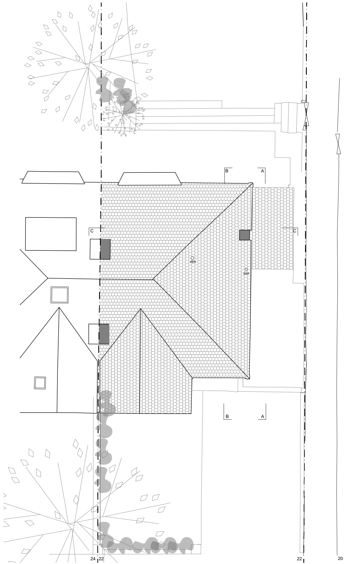
ROOF PLAN
