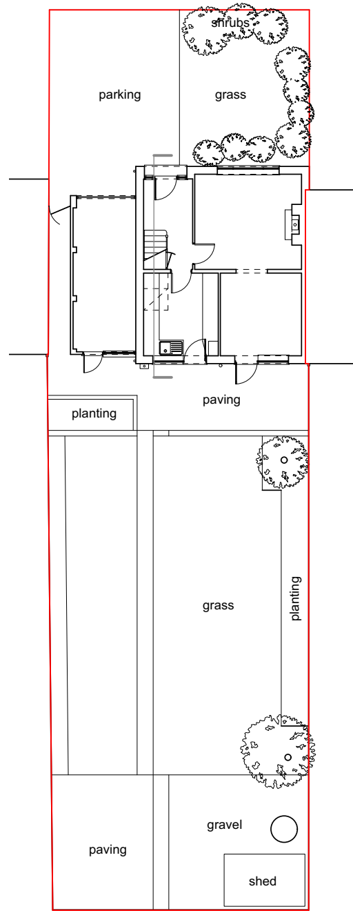
Existing Block Plan
