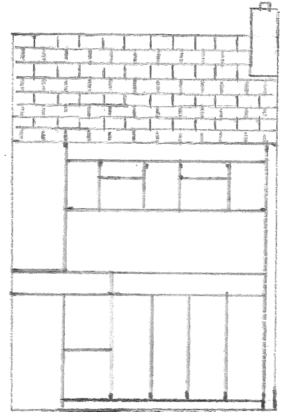
REAR ELEVATION
