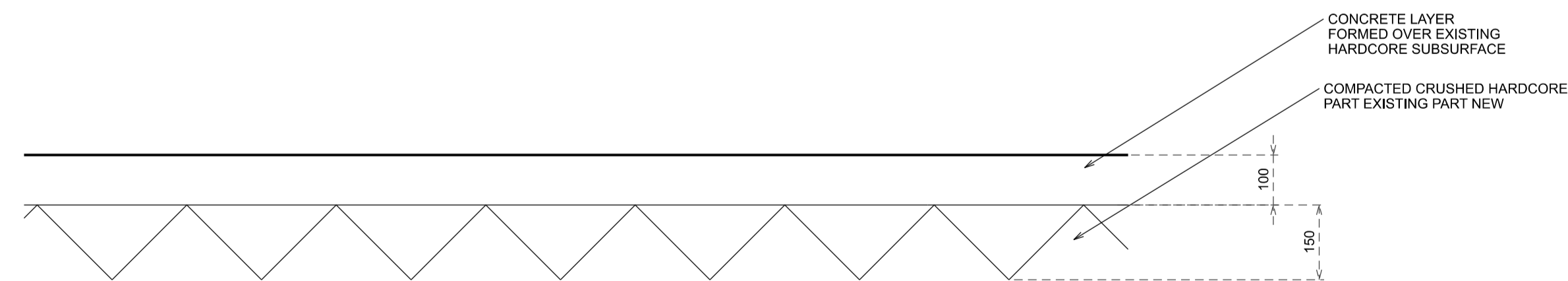
TYPICAL SECTION THROUGH HARDSTANDING (1:10)
