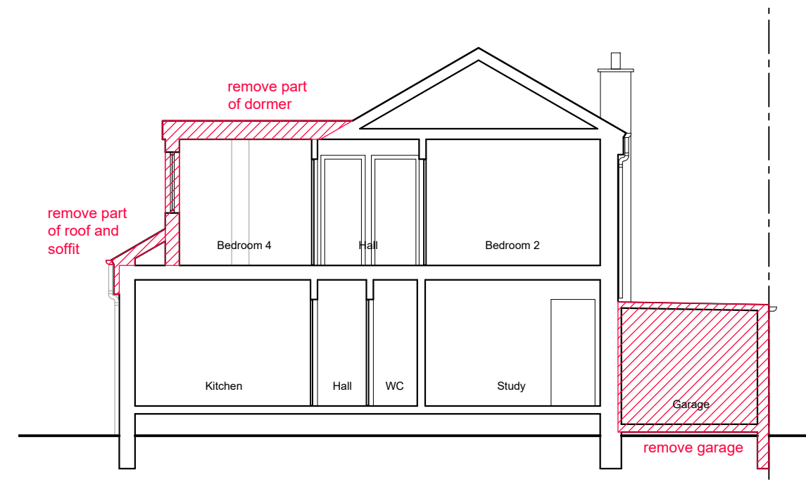
02 Section B-B' as existing 1:100 @ A3
