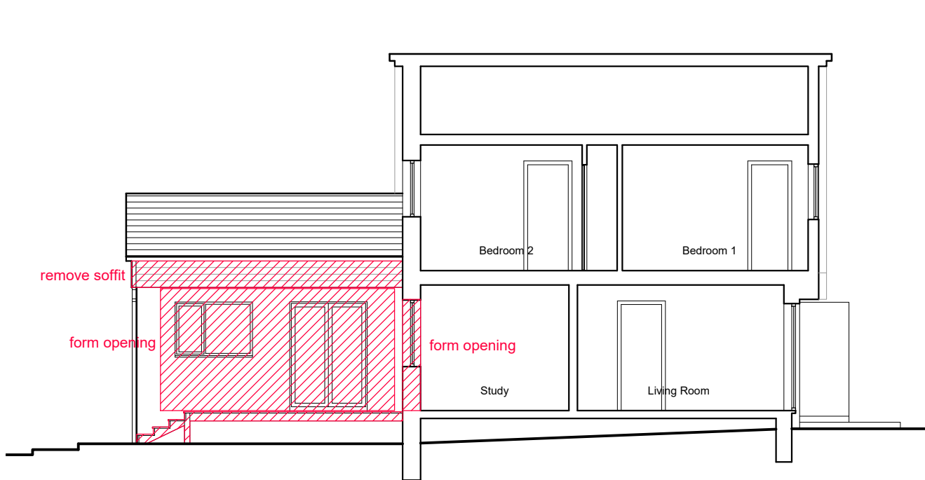
01 Section A-A' as existing 1:100 @ A3
