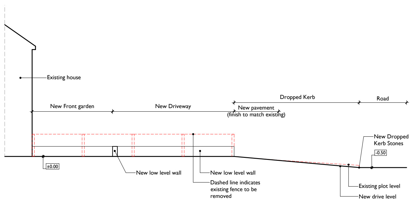
Proposed side boundary wall elevation
