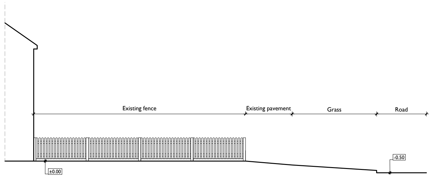
Existing side boundary wall elevation
