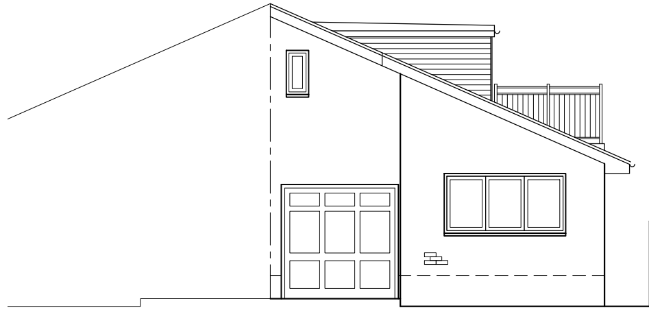
FRONT (N): EXISTING 1:100
