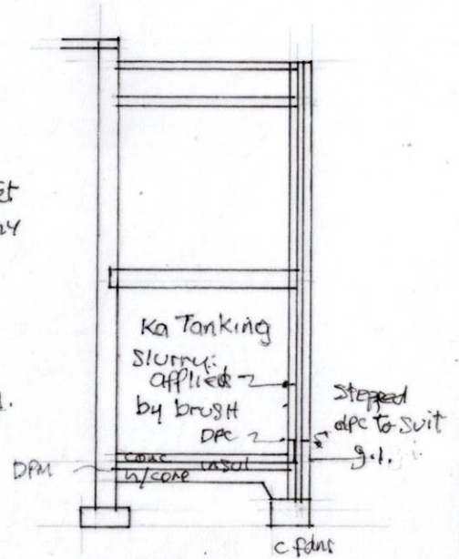
Section See Retaining wall Detail as below.
