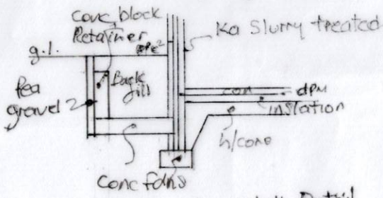
Retaining Wall Detail
