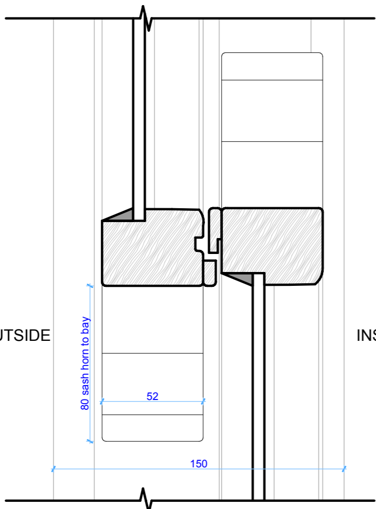
Detailed Section of Existing Typical Window Profile @ 1:2
