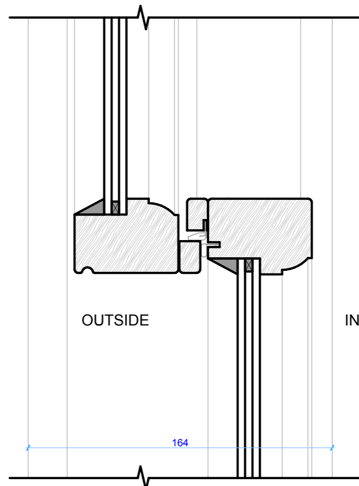
Detailed Section of Proposed Typical Window Profile @ 1:2
