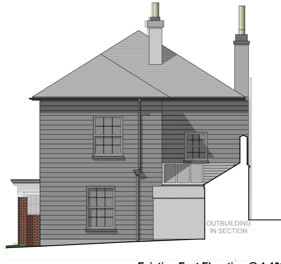
Existing East Elevation @ 1:100
