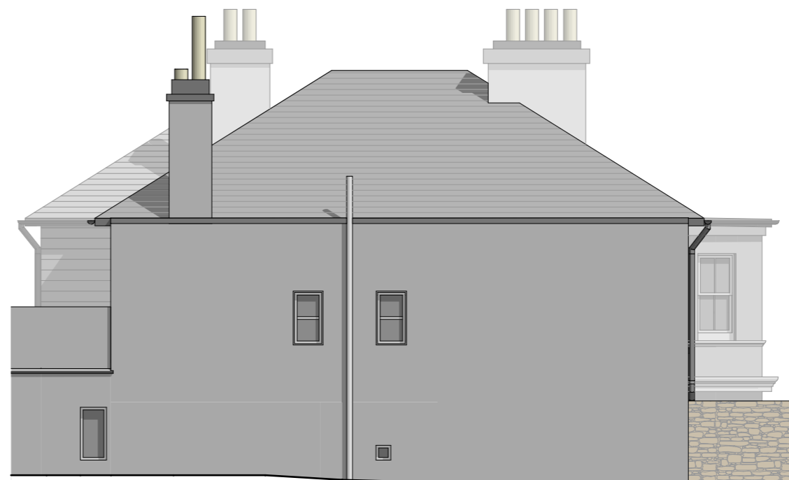
Existing North Elevation @ 1:100
