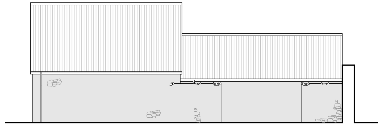
4 North East Elevation with Wall
