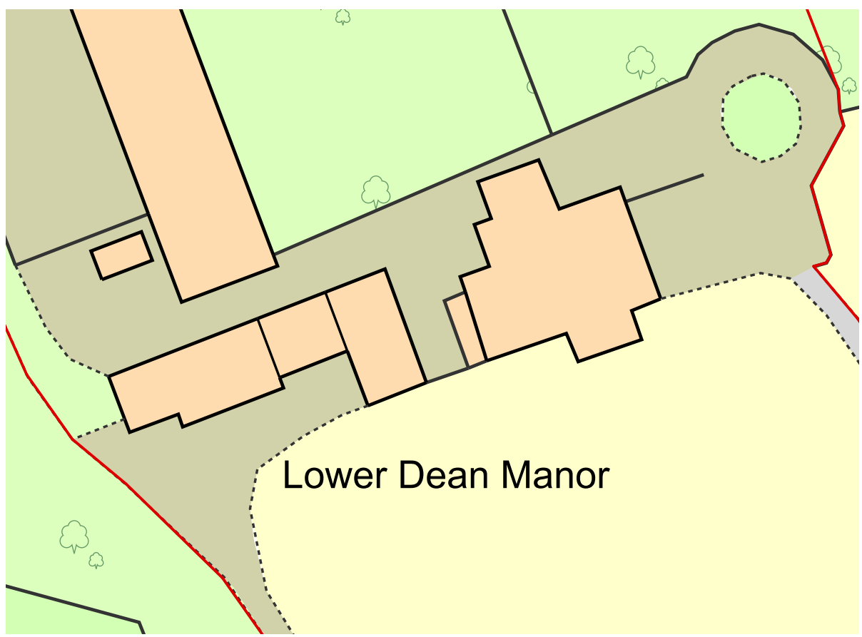
EXISTING BLOCK PLAN Scale: 1:500
