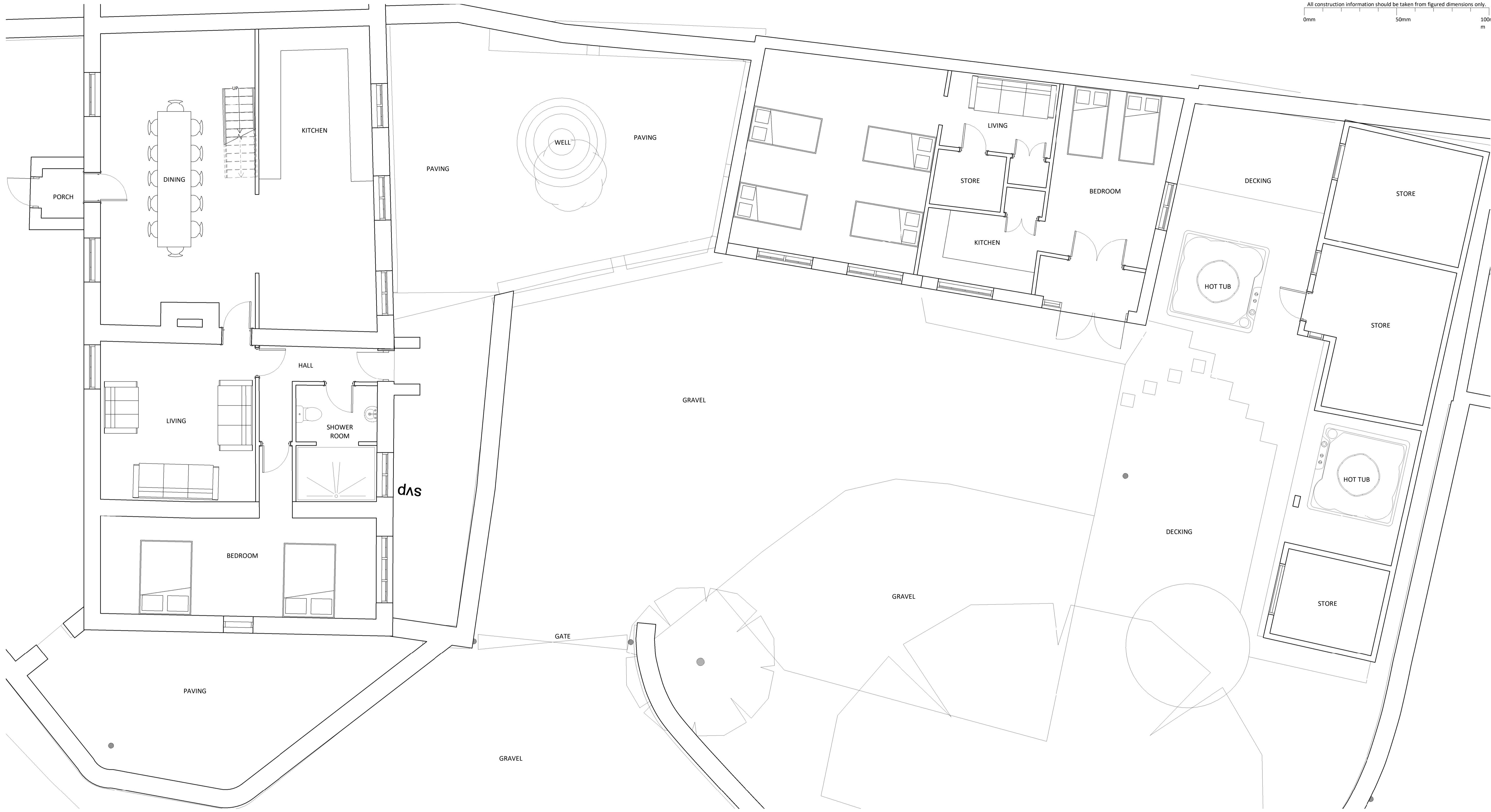
Linden Lodge Ground Floor Plan 1:50
