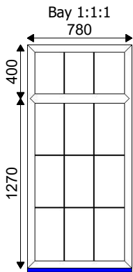
Bay 1:1:1 780 1-780x1700 C70 Case - White White 180mm Cill - White Drainage: CON 28mm Clear Geo bar A
