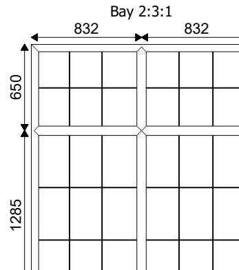
Bay 2:3:1 832 832 1-1664x1965 C70 Case - White White 180mm Cill - White Drainage: CON 28mm Clear Geo bar A
