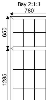
Bay 2:1:1 780 1-780x1965 C70 Case - White White 180mm Cill - White Drainage: CON 28mm Clear Geo bar A
