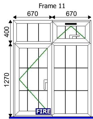
1-1340x1700 C70 Case - White White 180mm Cill - White Drainage: CON 28mm Clear Geo bar A
