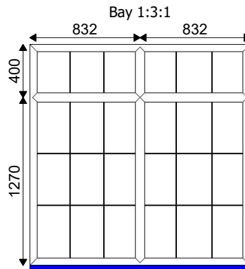
Bay 1:3:1 832 832 1-1664x1700 C70 Case - White White 180mm Cill - White Drainage: CON 28mm Clear Geo bar A
