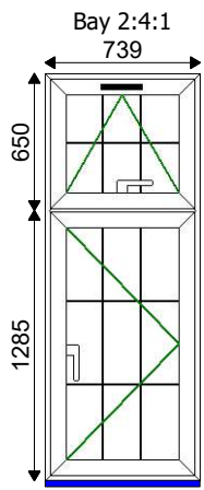
1-739x1965 C70 Case - White White 180mm Cill - White Drainage: CON 28mm Clear Geo bar A
