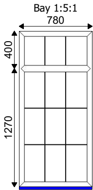
Bay 1:5:1 780 1-780x1700 C70 Case - White White 180mm Cill - White Drainage: CON 28mm Clear Geo bar A
