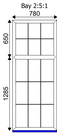
1-780x1965 C70 Case - White White 180mm Cill - White Drainage: CON 28mm Clear Geo bar A
