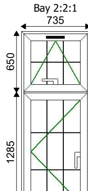
Bay 2:2:1 735 1-735x1965 C70 Case - White White 180mm Cill - White Drainage: CON 28mm Clear Geo bar A
