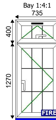
Bay 1:4:1 735 1-735x1700 C70 Case - White White 180mm Cill - White Drainage: CON 28mm Clear Geo bar A
